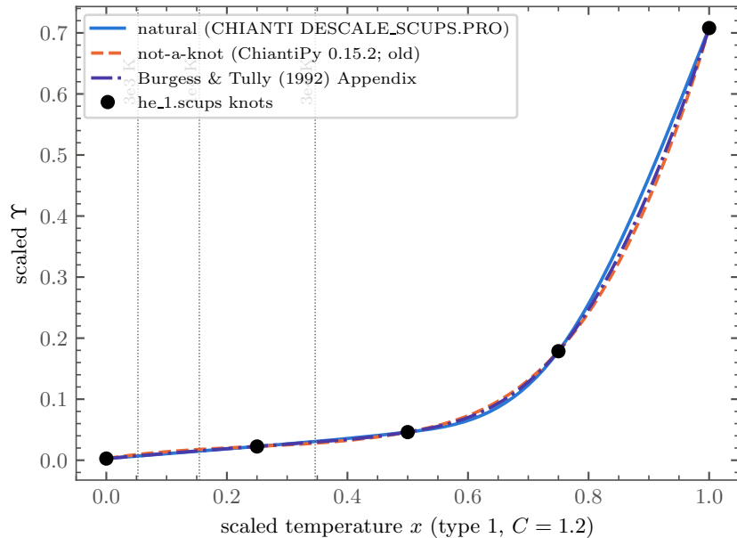
He I 1^1\text{S}-2^1\text{P}
