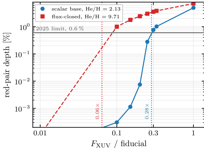
(b) the XUV the 2025 non-detection allows
