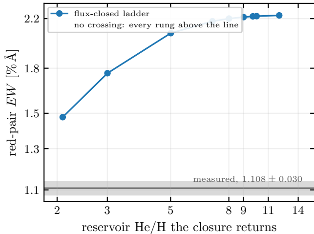
(a) what the closed composition gives
