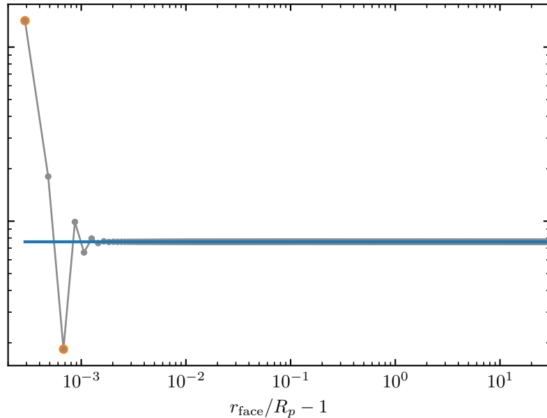
LHS 1140 b, K_{zz} = 10^9 , He/H 1.8
