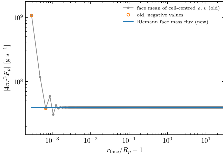
LHS 1140 b, K_{zz} = 10^9 , He/H 0.55
