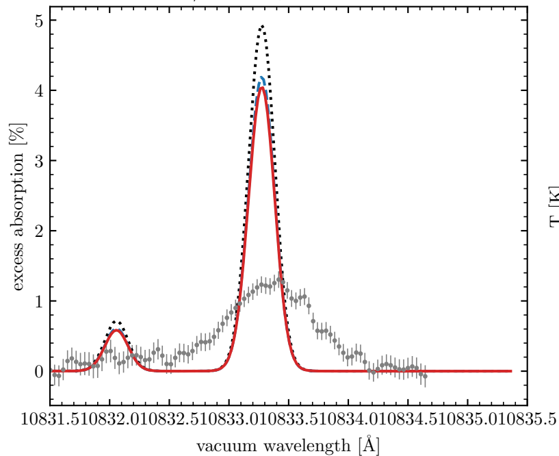
He/H = 1.8, unbroadened
