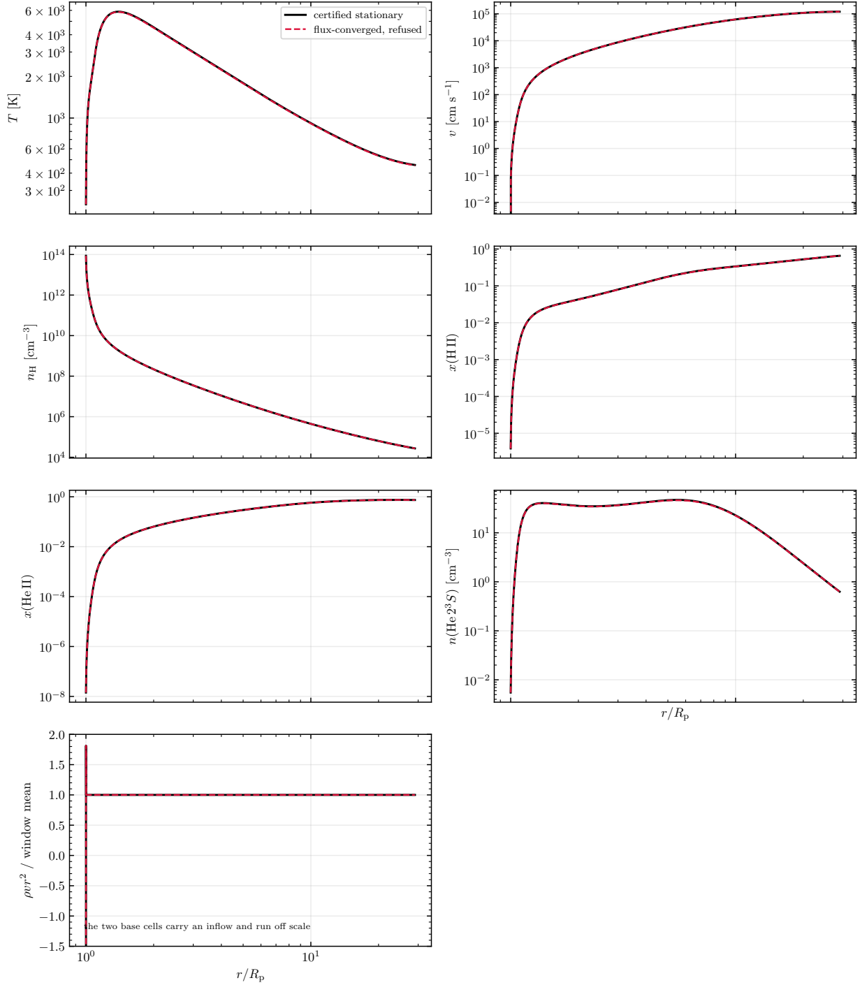
Figure 4: The certified stationary solution and the flux-converged refused state of the atomic scalar_gj1132_kzz1e9/HeH2.13, as functions of radius.
