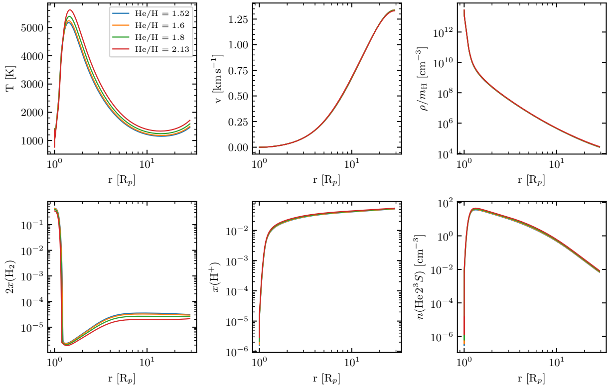
Figure 3: The certified molecular K_{zz} = 10^9 states \text{He}/\text{H} = 1.52 to 2.13 under the corrected atomic physics (advection-corrected profiles): temperature, velocity, \rho/m_{\text{H}} , \text{H}_2 fraction, \text{H II} fraction and n(\text{He } 2^3\text{S}) against radius.
