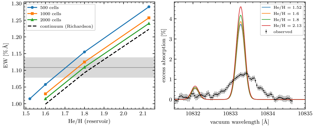
Figure 1: Left: the red-pair EW of the certified molecular states against the reservoir He/H on 500, 1000 and 2000 cells and in the continuum limit, with the observed 1.108 \pm 0.030 % Å (grey). Right: the unbroadened 500-cell spectra against the released one.
