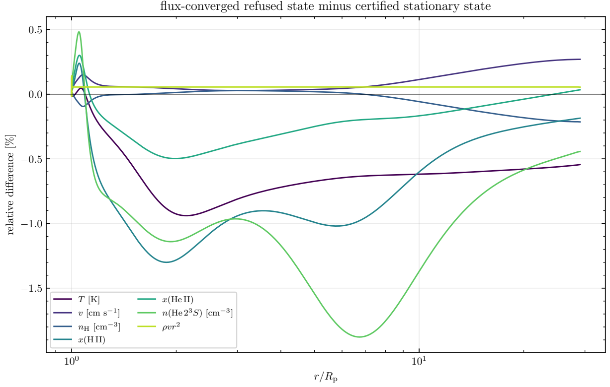
Figure 5: The same two states, as the relative difference of each quantity. The largest are the temperature at r = 2.13 R_p ( -0.94 per cent), x(\text{H II}) at 1.87 ( -1.30 ) and n(\text{He } 2^3S) at 6.74 ( -1.88 ).
