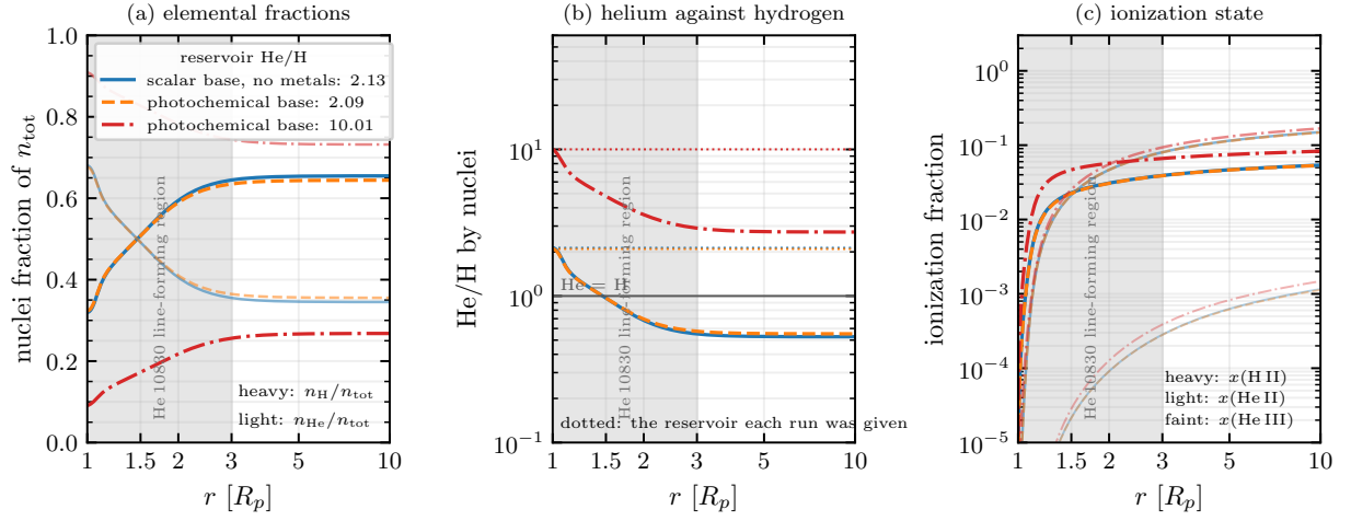
Figure 16: Composition and ionization against radius, for the three solutions of Table 15, from the same advection-corrected profiles. (a) the hydrogen and helium nuclei fractions of n_{\text{tot}} ; (b) He/H by nuclei, with the reservoir each run was given as a dotted line, so the vertical drop from dotted line to curve is what element diffusion does; (c) the ionization fractions. n_{\text{tot}} counts one particle per species, H I, H II, He I, He II, He III and every metal ion stage, with electrons excluded, and He 2^3S not added because it is an excited level inside He I, so (a) does not sum to one on the photochemical base. The metals it misses are negligible: their largest share of n_{\text{tot}} anywhere in 1–30 R_p is 2.3 \times 10^{-4} at He/H = 2.09 and 9.7 \times 10^{-5} at 10.01, and zero on the metal-free base. Nuclei are counted as H I + H II and He I + He II + He III. The flux-consistent sequence does not cross the measurement anywhere (Sect. 12.7), so no crossing is marked between the two profile runs drawn here. The He 10830 line-forming region 1–3 R_p is shaded.
