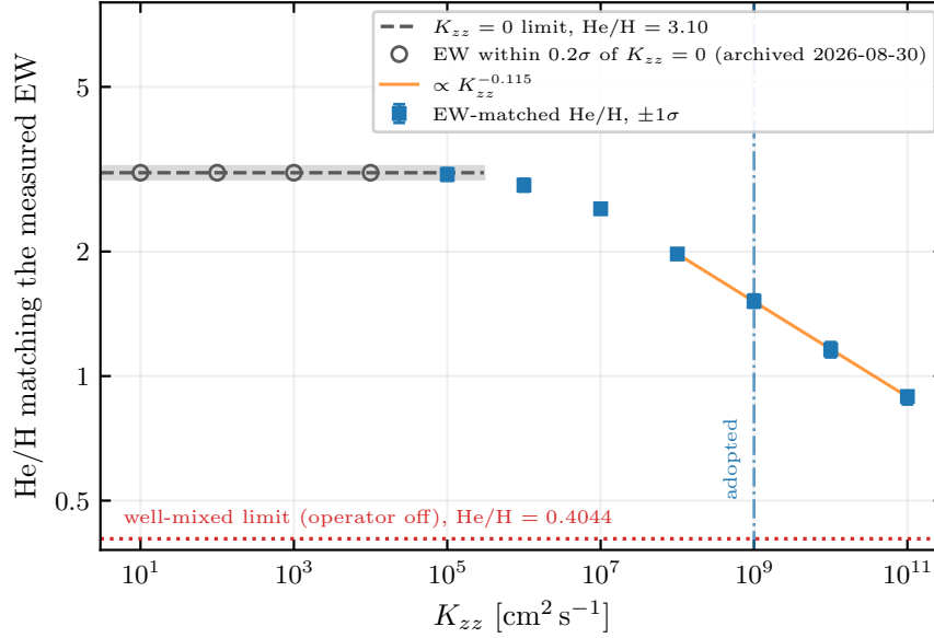
Figure 6: The composition–mixing degeneracy in full. Each square is the He/H reservoir ratio whose red-pair equivalent width equals the measured one, solved at one decade of K_{zz} with helium and hydrogen free to separate by diffusion (Table 5); the error bars propagate the measurement error alone and are smaller than the symbols over most of the range. The landscape has three parts. Below K_{zz} \simeq 10^5 the eddy term is a small correction to the molecular coefficient the base already carries, the inference sits on a plateau at He/H = 3.10 (dashed, with its 1\sigma band), and the open circles mark the decades whose equivalent width, on the 2026-08-30 solutions, differed from the K_{zz} = 0 one by less than a fifth of the measurement error. Between 10^6 and 10^7 the curve rolls off. From 10^8 up it is the shallow power law K_{zz}^{-0.115} (orange, fitted to those four points). Neither end of the axis reaches the well-mixed crossing of 0.4044 (dotted): with diffusion active, helium settles at every eddy coefficient tried, and He/H inferred from this line is a statement about the assumed mixing as much as about the planet. The adopted K_{zz} = 10^9 \text{ cm}^2 \text{ s}^{-1} is marked.
