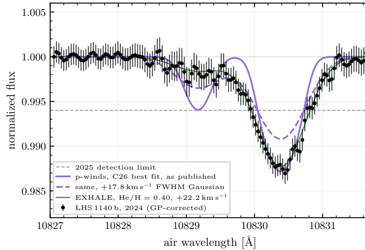
Figure 9: The C26 p-winds best fit as published (solid purple) and convolved with the 17.8 \text{ km s}^{-1} FWHM Gaussian that reproduces the measured width (dashed purple), against the measurement. The EXHALE \text{He}/\text{H} = 0.40 curve at its own matched Gaussian ( 22.2 \text{ km s}^{-1} , thin green) is repeated from Fig. 5. Broadened to the observed width, the p-winds curve passes above the red core, so the width is matched and the depth is not. All curves are shifted by the same v_{\text{wind}} = +2.26 \text{ km s}^{-1} .
