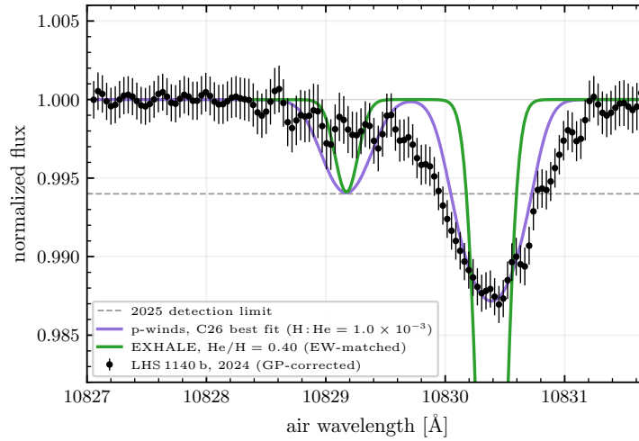
Figure 11: The two best models over the 2024 spectrum, in the presentation of the paper’s Fig. 4: p-winds at the C26 best fit (the MCMC medians) with the authors’ settings, and EXHALE at the composition matched on equivalent width, \text{He}/\text{H} = 0.40 . Both are shifted by the fitted v_{\text{wind}} = +2.26 \text{ km s}^{-1} .
