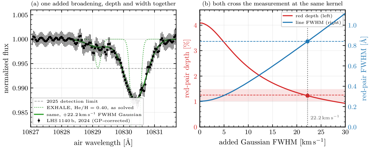
Figure 5: Left: the EXHALE profile matched on equivalent width as solved (dotted, its core running below the plotted range) and convolved with a 22.22 \text{ km s}^{-1} FWHM Gaussian (solid), against the measurement. Both are shifted by the same v_{\text{wind}} = +2.26 \text{ km s}^{-1} used in the earlier figures. Right: red-pair depth (red, left axis) and red-pair FWHM (blue, right axis) as the added Gaussian is scanned. Dashed lines are the observed values, the shaded band the C26 1\sigma interval on the depth; the dotted vertical marks where the width is matched. Both curves meet the measurement at the same Gaussian.
