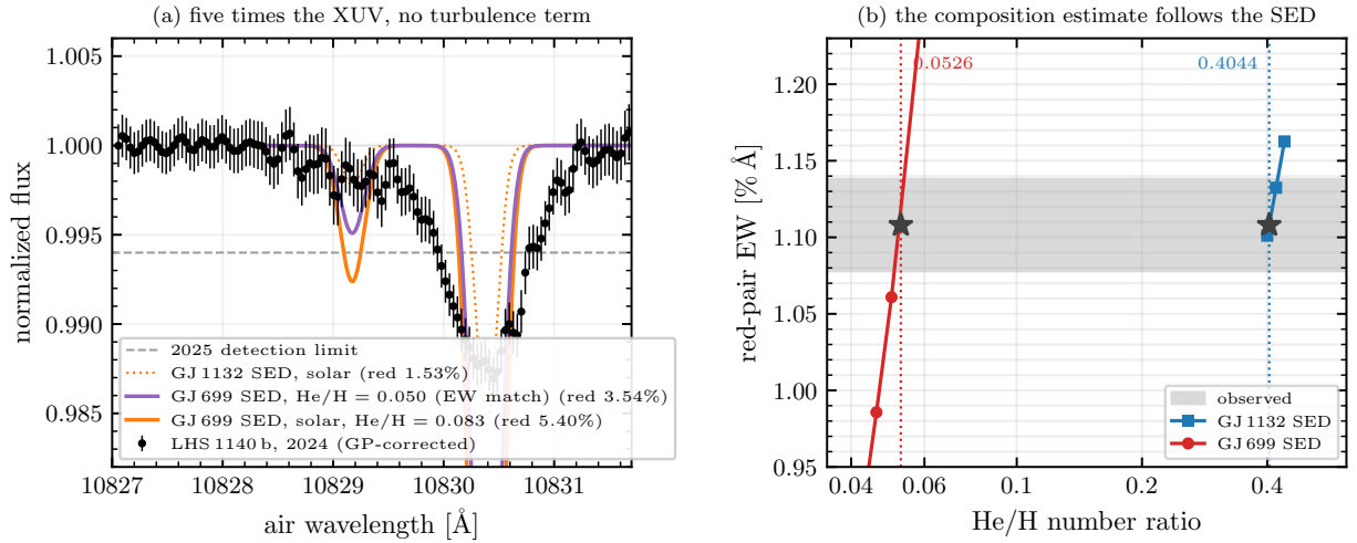
Figure 13: The GJ 699 proxy, five times the XUV of the GJ 1132 proxy used elsewhere in this memo. Left: the measurement with the EXHALE solution nearest the equivalent-width crossing 0.0526 , the one at \text{He}/\text{H} = 0.050 , and the solar case on this spectrum, with the GJ 1132 solar case dotted for contrast; all curves without the turbulence term and shifted by the fitted v_{\text{wind}} = +2.26\text{ km s}^{-1} . The lines are deeper but no wider, the GJ 699 solar curve reaching 3.5\times the depth of the GJ 1132 one ( 5.40\% against 1.53\% ) while the added broadening the measurement demands of the two differs by 0.45\text{ km s}^{-1} , or 2 per cent ( 21.95 against 22.40\text{ km s}^{-1} ). Right: red-pair equivalent width against composition for the two spectra, with the measured band and the two crossings; the composition the line implies moves from 0.4044 to 0.0526 when the assumed spectrum is changed.
