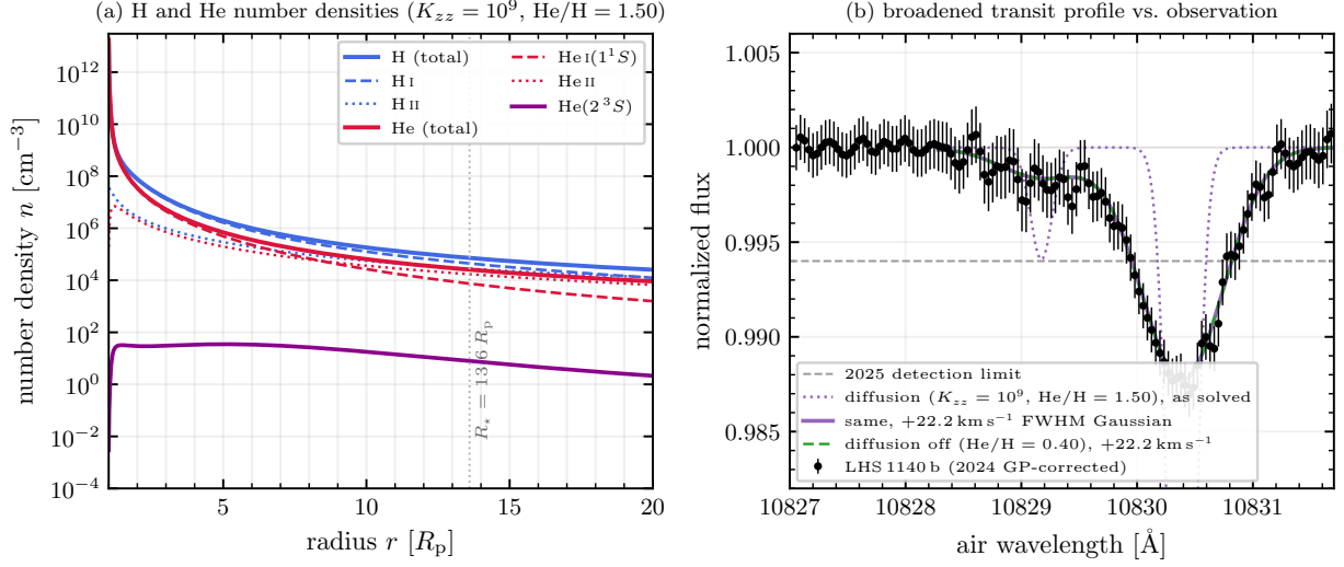
Figure 8: The diffusive solution matched on equivalent width ( \text{He}/\text{H} = 1.50 at K_{zz} = 10^9 \text{ cm}^2 \text{ s}^{-1} ). (a) Absolute number densities of hydrogen species (total H, H I, H II) and helium species (total He, He I( 1^1S ), He II, and metastable He( 2^3S )) as a function of planetary radius r [ R_p ]. At the lower boundary ( r = 1.0 R_p ), \text{He}/\text{H} = 1.50 ; diffusion lets helium settle outward relative to hydrogen, with the local abundance falling to \text{He}/\text{H} = 0.456 at 2 R_p and 0.355 at 10 R_p . Dotted vertical line marks the stellar disk radius ( 13.6 R_p ). (b) The transmission spectrum as solved (dotted purple, its core running below the plotted range) and convolved with the 22.22 \text{ km s}^{-1} FWHM Gaussian that reproduces the measured width (solid purple), against the measurement; the well-mixed curve solved without diffusion, at its own matched Gaussian (dashed green), is repeated from Fig. 5. The two broadened curves are indistinguishable: their Gaussians agree to four digits. All model curves are shifted by the fitted v_{\text{wind}} = +2.26 \text{ km s}^{-1} .
