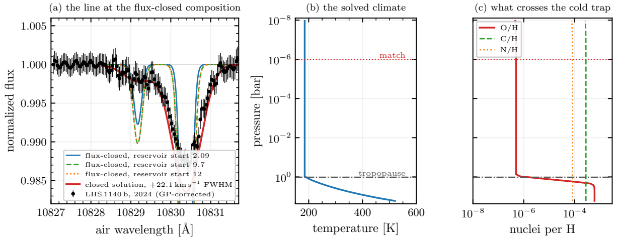
Figure 19: The flux-consistent solutions and the column they stand on. (a) Three of them (started at reservoirs 2.09, 9.7 and 12) against the measurement; the thick curve is the lowest of them convolved with the 22.1 km s -1 FWHM Gaussian that reproduces the observed width, which then lands below the observed flux because the equivalent width was already 33 per cent too large. Model curves are shifted by the fitted v_{\text{wind}} = +2.26 km s -1 , as elsewhere in this memo. (b) The solved climate of the column handed over, with the tropopause at 1.031 bar and the 1 μbar matching level marked; the stratosphere sits at the skin temperature, 185 K. (c) The elemental abundances the profile carries. Oxygen is cut by a factor 1223 at the tropopause by the water cold trap, while carbon and nitrogen cross it unchanged. On the current C, N and O cooling those elements no longer weaken the line (Sect. 2.4); on the 2026-08-30 solutions they made it 2.6× weaker than the metal-free base at the same reservoir. Panels (b) and (c) place the column in the iteration; every column of the file itself is in Figs. 14 and 15.
