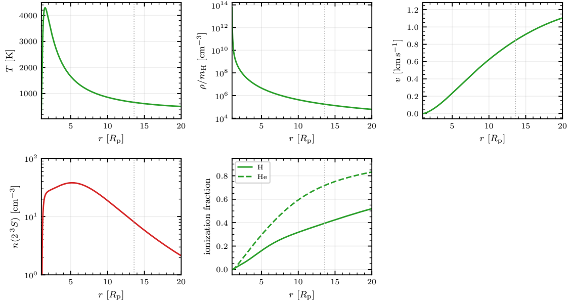
Figure 12: The EXHALE solution matched on equivalent width (the solved composition \text{He}/\text{H} = 0.40 , nearest the well-mixed crossing at 0.4044): temperature, density, velocity, metastable helium density, and ionization fractions. Dotted vertical line: the stellar radius.
