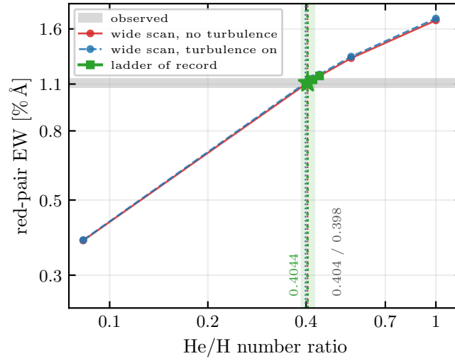
Figure 4: Red-pair equivalent width against composition, with and without the turbulence term, compared with the measured band. The crossing is insensitive to the broadening treatment: each solved composition of the well-mixed group up to \text{He}/\text{H} = 1 carries both syntheses of the same solution, so the two curves differ only in the broadening, and they cross the measured band at \text{He}/\text{H} = 0.4044 without the turbulence term and 0.3985 with it, 1.5 per cent apart. The three compositions 0.40, 0.42 and 0.44 drawn on top are where the spacing brackets the measurement directly.
