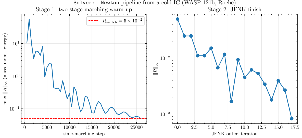
Figure 1: The Solver: Newton route from a cold IC (WASP-121b, Roche). Left: maximum steady residual \max \|R\|_\infty over the mass, momentum, and energy equations during the two-stage (Reconstruction scheme: PLM+WENO3) marching warm-up; the dashed line is the legacy residual hand-off threshold R_{\text{switch}} = 5 \times 10^{-2} used when this figure was produced (the current default keys the hand-off on du < 10^{-2} instead, at a comparable point on the warm-up). Right: residual vs. JFNK outer iteration during the Newton finish, down to Resid tol ( 10^{-5} ).
