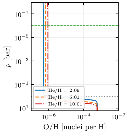
(f) the cold trap, by reservoir
