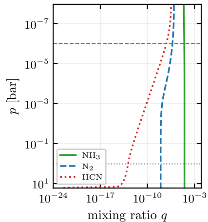
(f) the cold trap, by reservoir
