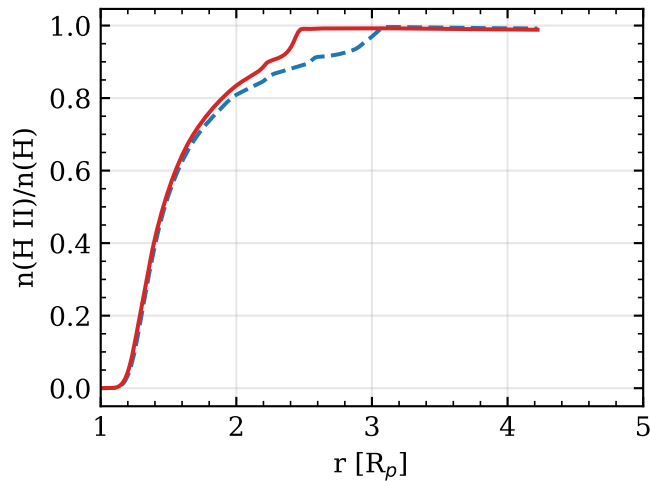
H ionization fraction
