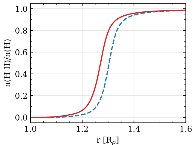
H ionization fraction
