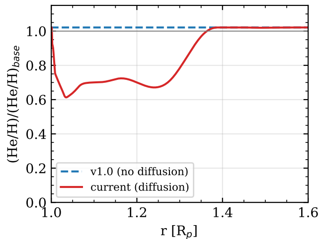
He/H element ratio
