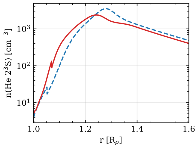
metastable He 2^3\text{S}
