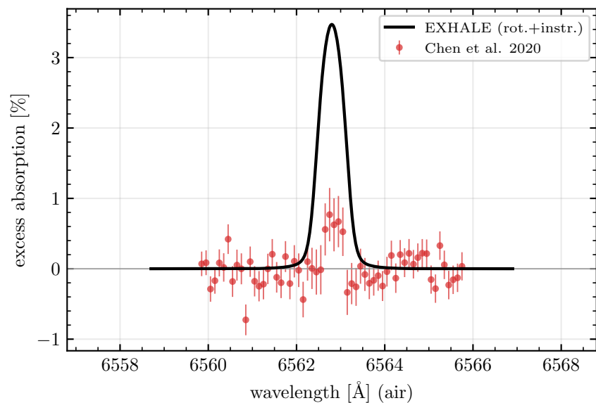
WASP-52 b
