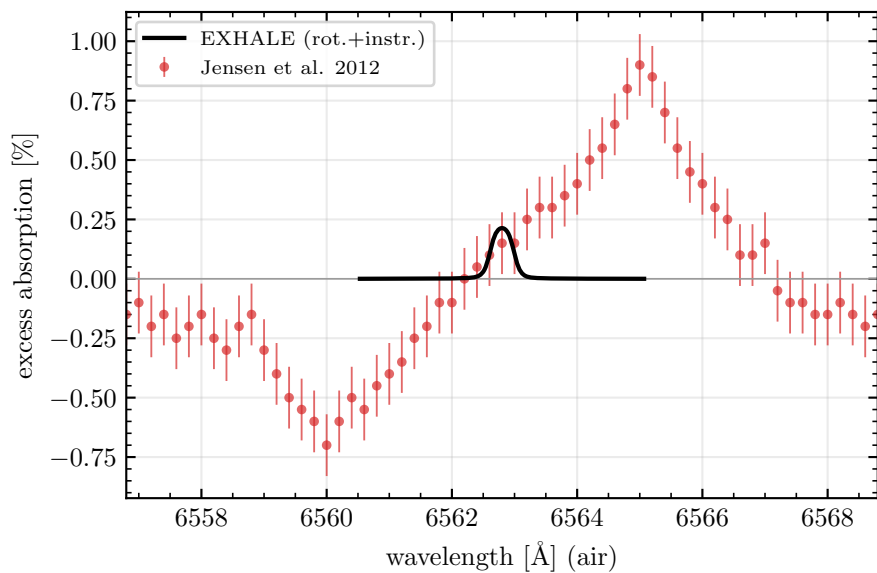
WASP-52 b
