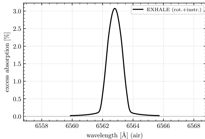
WASP-121 b
