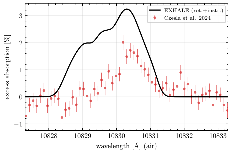
WASP-121 b
