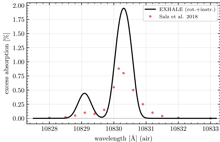
WASP-121 b
