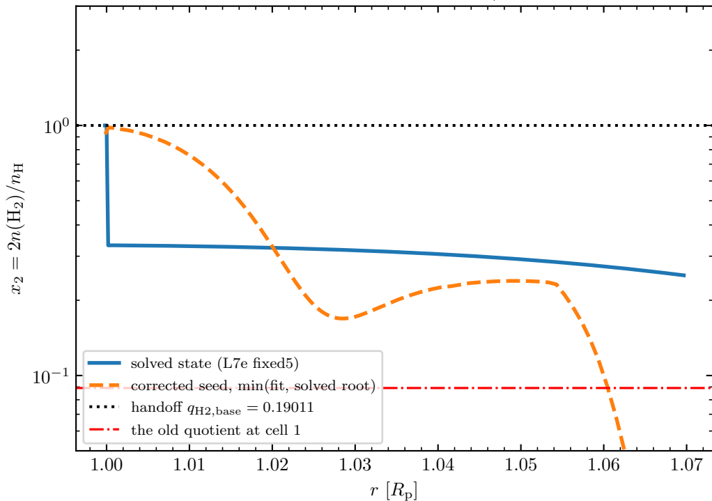
Base layer H 2 , LHS 1140 b, He/H = 2.13
