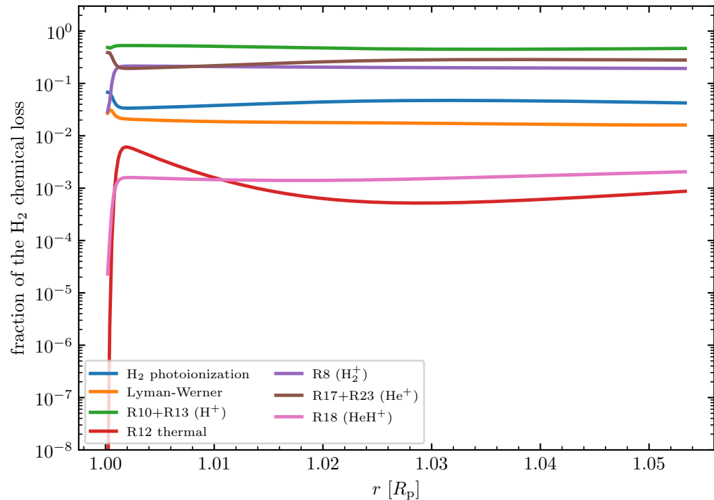
What destroys H 2 through the layer
