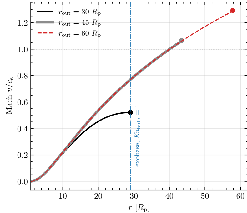
Mach number of the solved state
