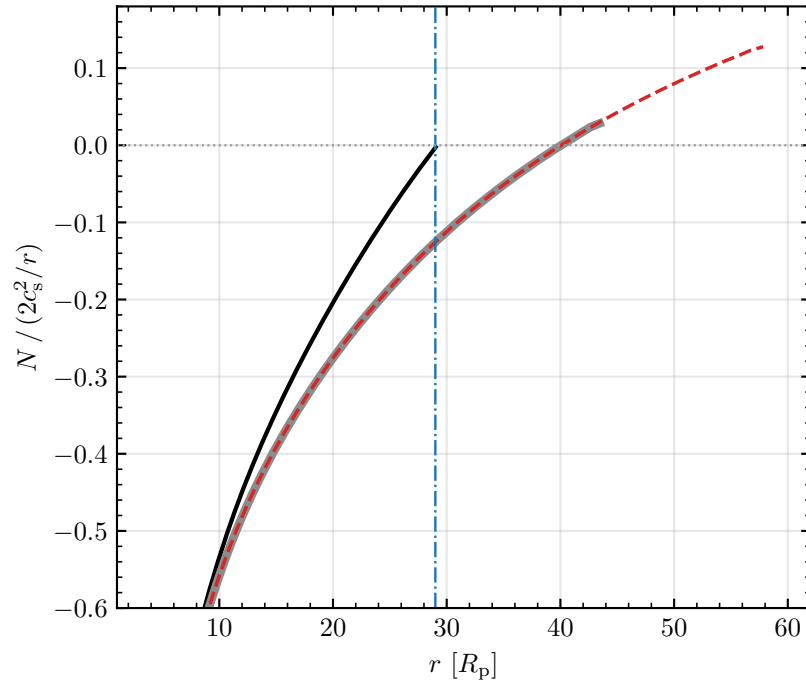
N = 2c_s^2/r - GM/r^2 - (\gamma - 1)q/v
