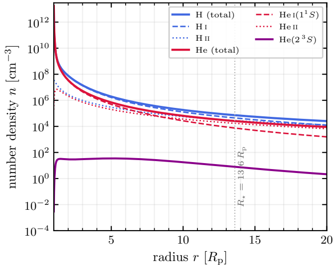
(a) H and He number densities ( K_{zz} = 10^9 , He/H = 1.50)
