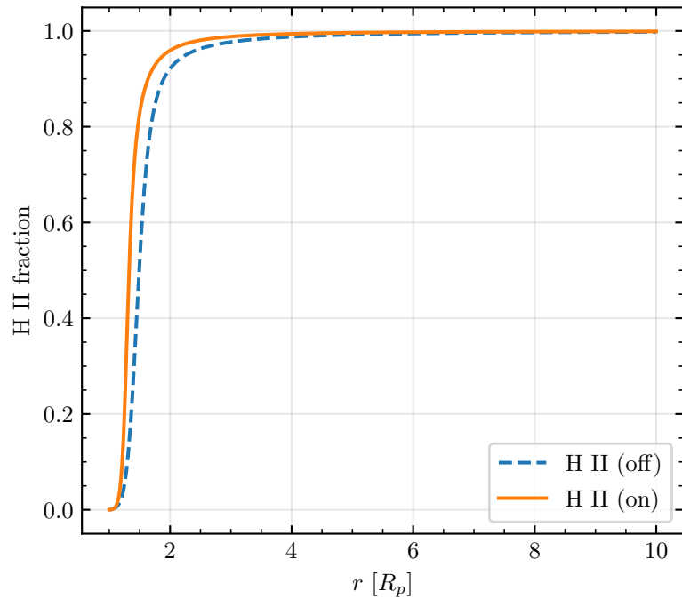
while the H ionization is barely affected
