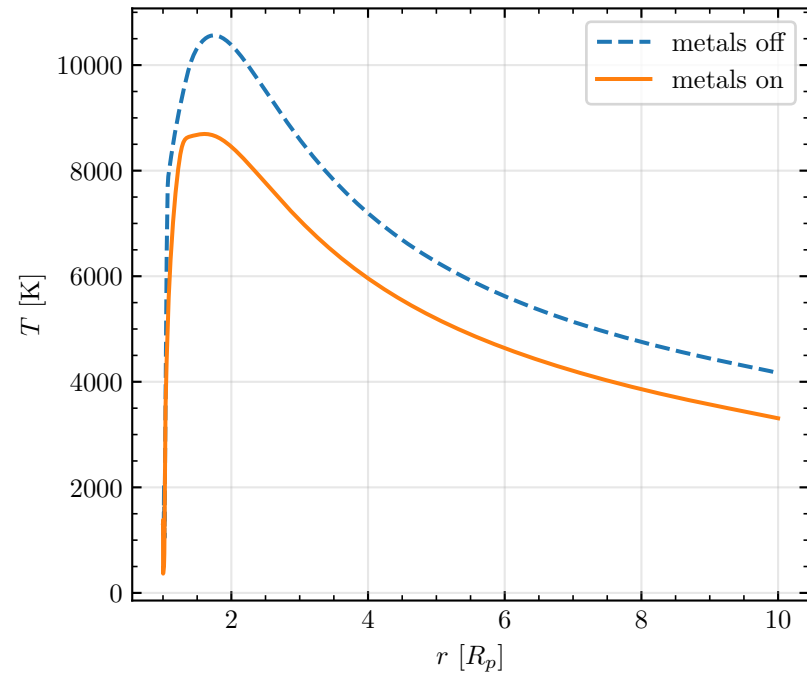
Metal-line cooling lowers the peak temperature
