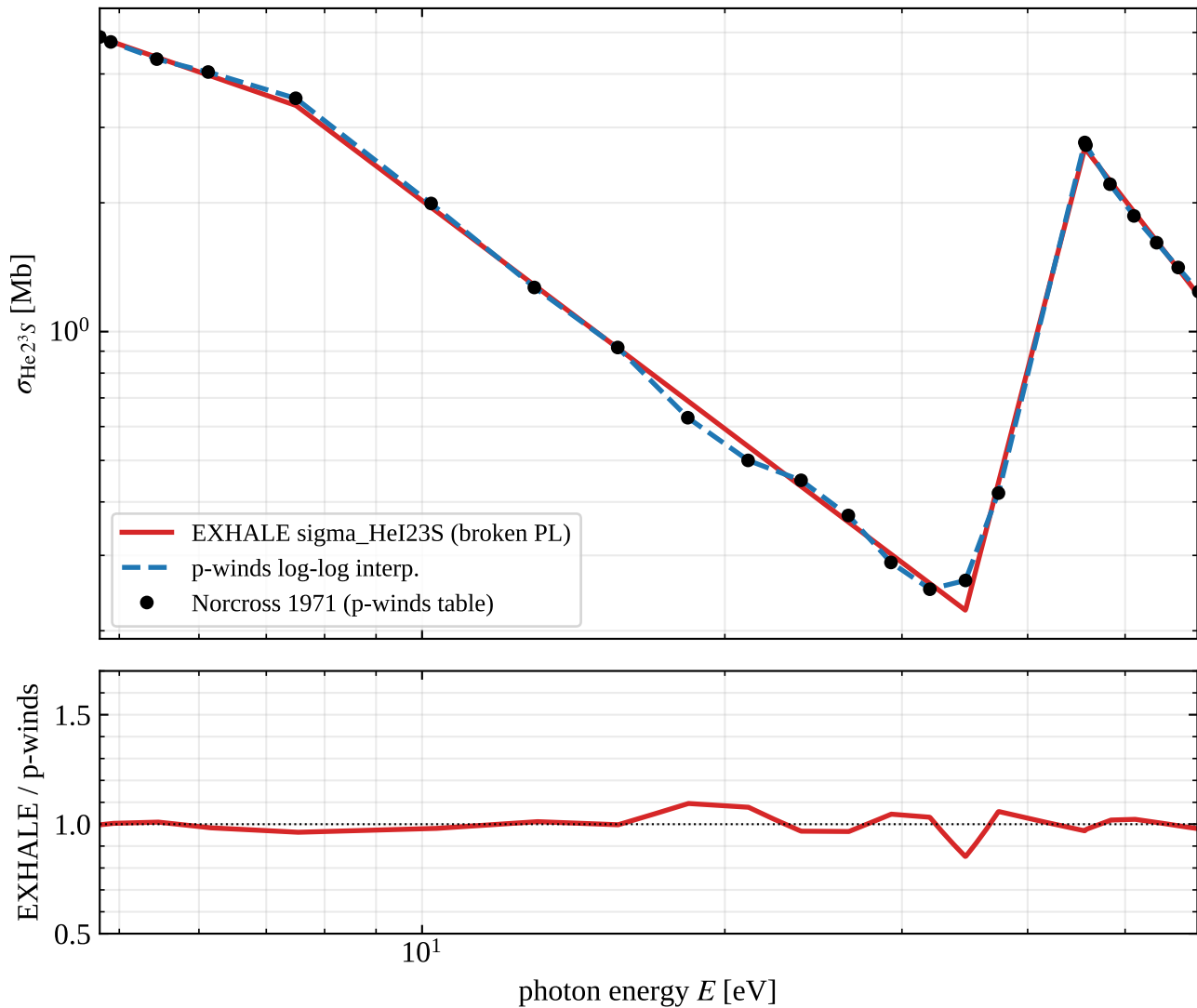
He I 2^3\text{S} photoionization: EXHALE vs p-winds (Norcross 1971)
