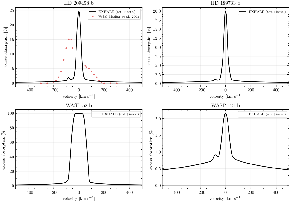
Figure 7. Synthetic Ly \alpha transit spectra on a velocity axis, as in Figure 5. The HD 209458 b panel overplots the wing profile of A. Vidal-Madjar et al. (2003); the line core (roughly \pm 40 km s ^{-1} ) is omitted in the data because of interstellar and geocoronal absorption. No Ly \alpha measurements are available for the other three planets. Generated by python/make_transit_figures.py .
