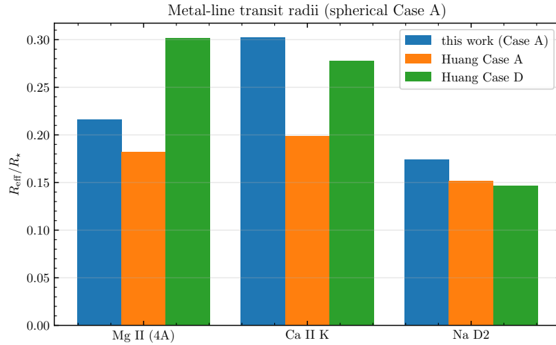
Figure 7: Metal-line transit radii R_{\text{eff}}/R_\star for spherical Case A, compared with Huang et al. (2023) Case A and Case D.
