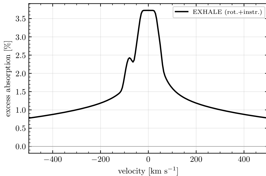
WASP-121 b
