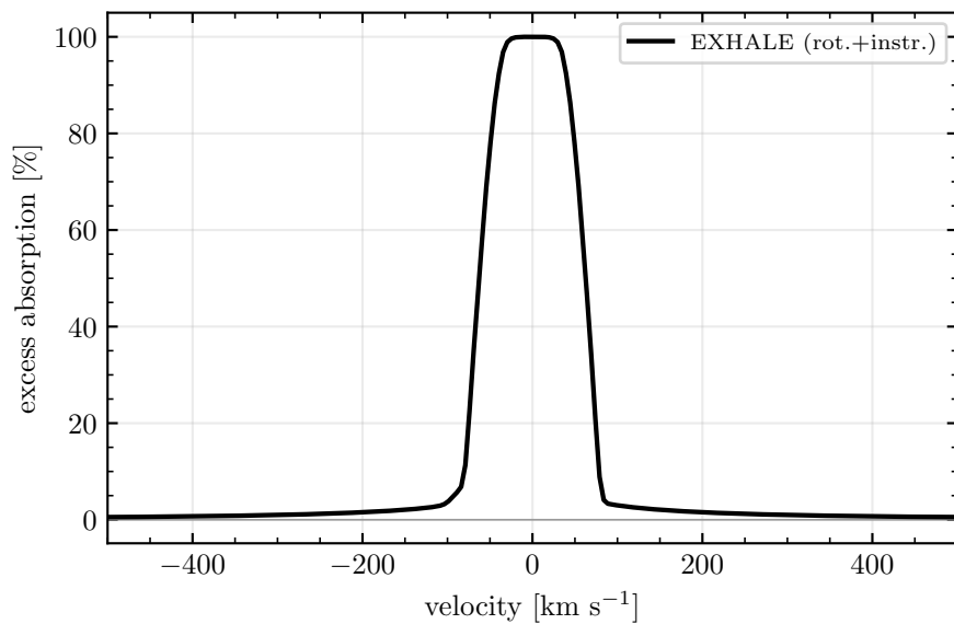
WASP-52 b
