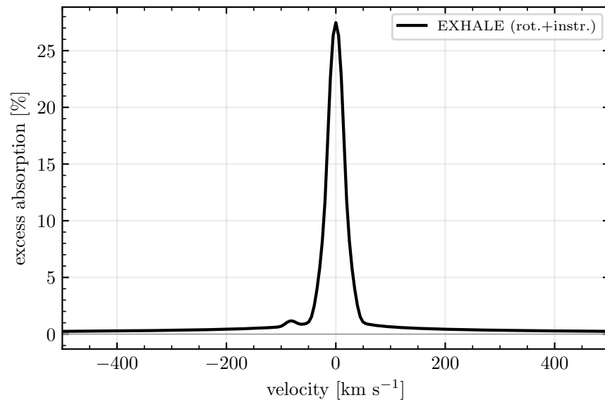
WASP-121 b
