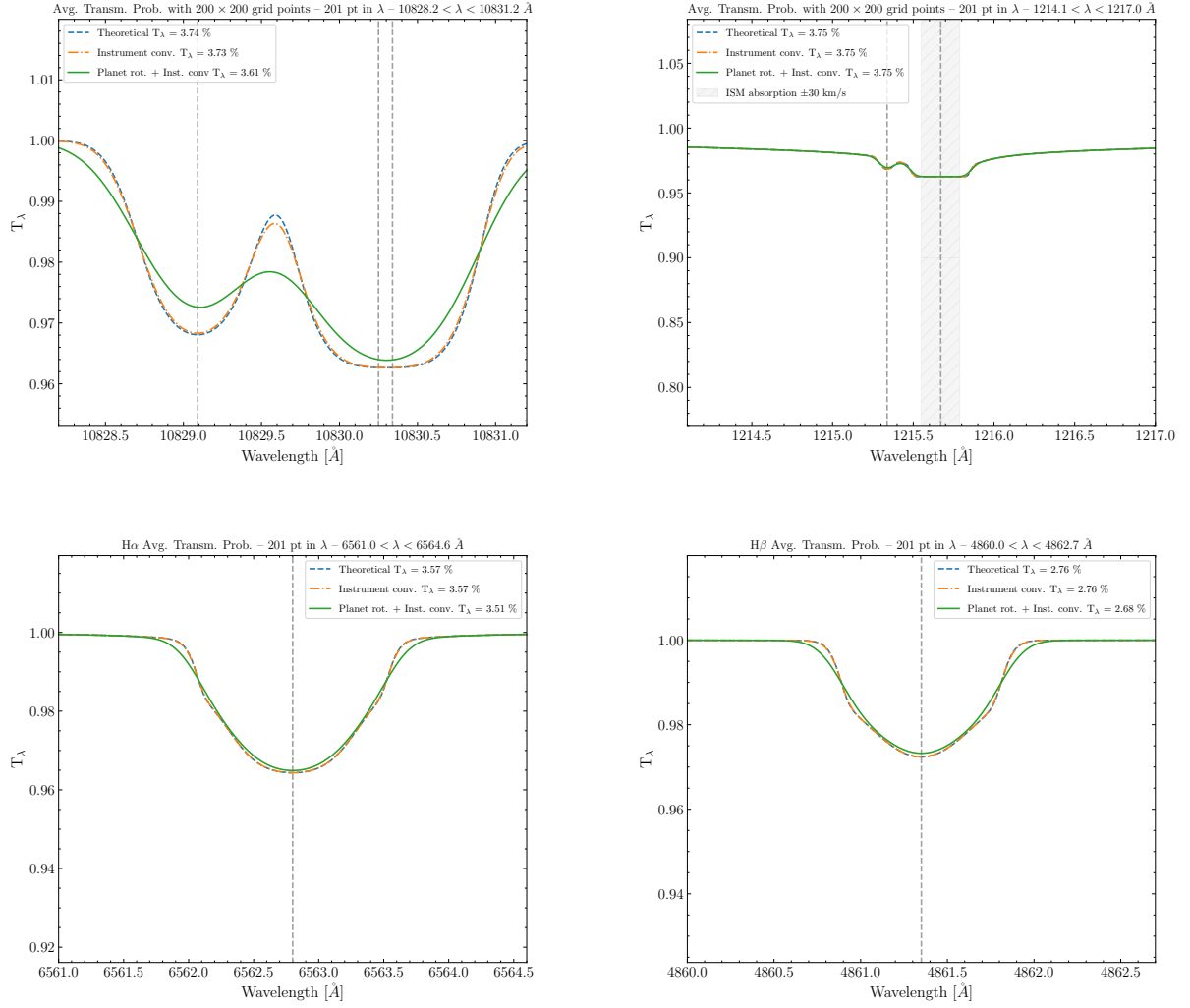
Figure 2: EXHALE_transit.py output spectra for WASP-121b (Roche, Newton solution with He 2 3 S on; backup/regression/tpm_wasp/): HeI 10830 (top left), Ly \alpha (top right), H \alpha (bottom left), and H \beta (bottom right). Each panel shows the theoretical line, the instrument-convolved line, and the instrument+rotation-convolved line as produced by the script.
