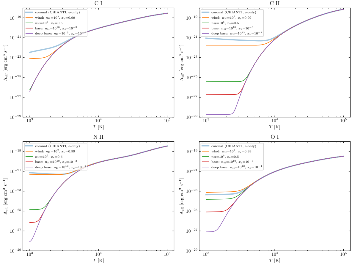
Figure 4: Effective CI, CII, NII and OI cooling coefficients with the ground term solved in statistical equilibrium, Eqs. (5) and (7), for densities from the wind to the deep base, compared with the electron-only coronal curve. The low-temperature plateau of each coronal curve is the unsaturated fine-structure floor; it collapses by several decades once the ground term is allowed to thermalise.
