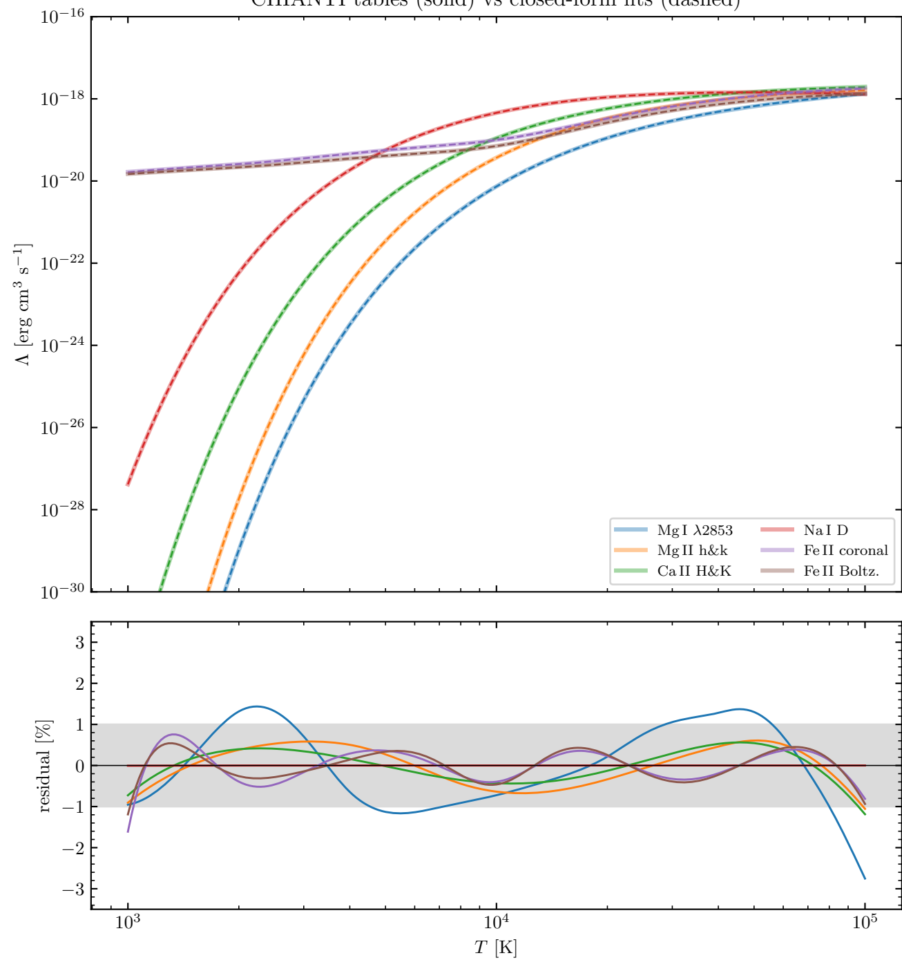
CHIANTI tables (solid) vs closed-form fits (dashed)
