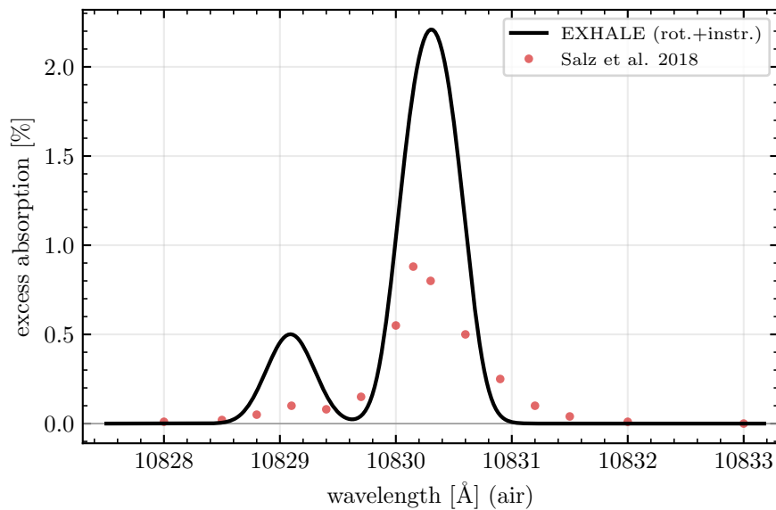
WASP-121 b
