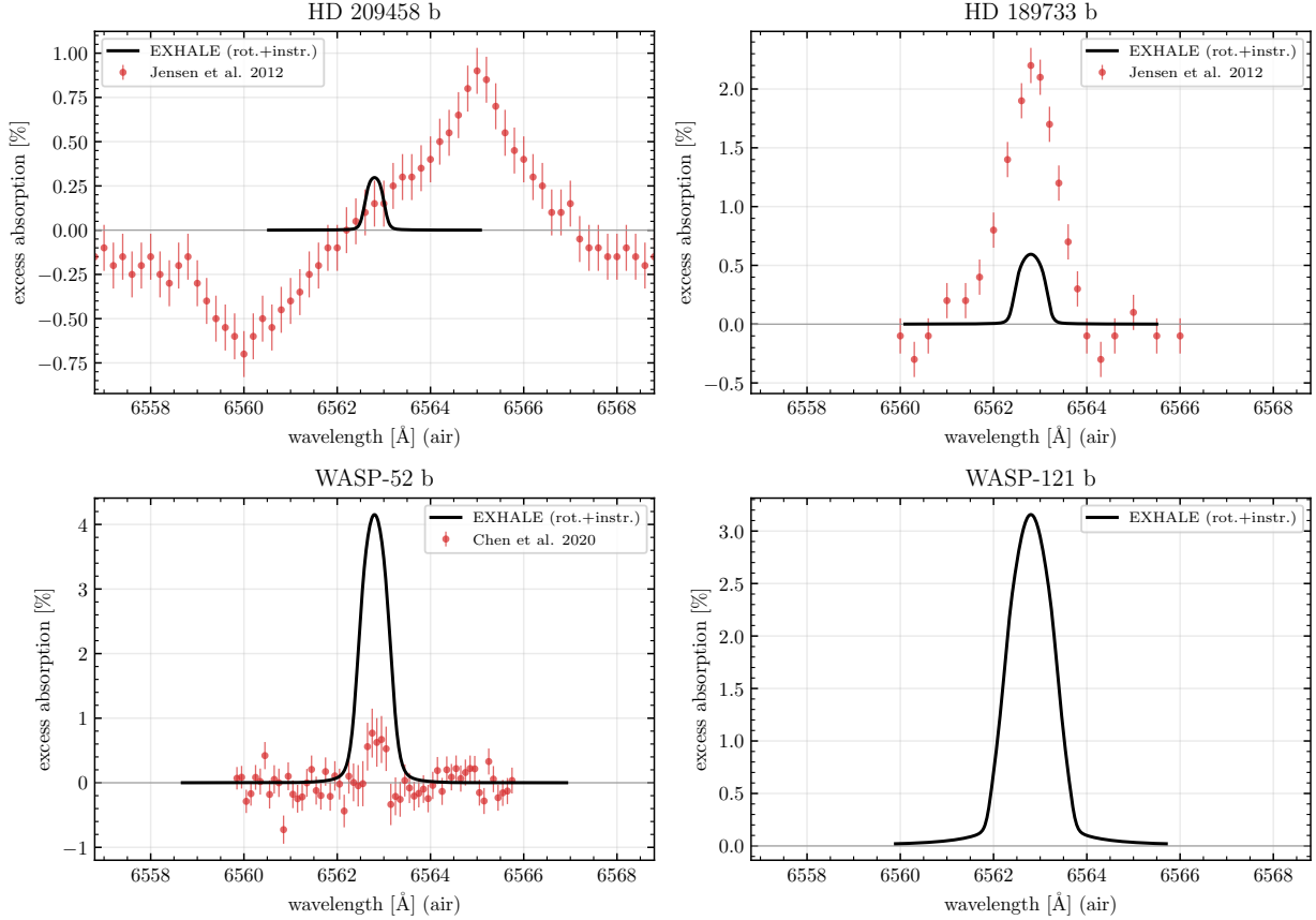
Figure 6. Synthetic \text{H}\alpha transit spectra, as in Figure 5, compared with the digitized A. G. Jensen et al. (2012) traces (HD 209458 b and HD 189733 b) and the G. Chen et al. (2020) ESPRESSO spectrum (WASP-52 b). Generated by python/make_transit_figures.py .
