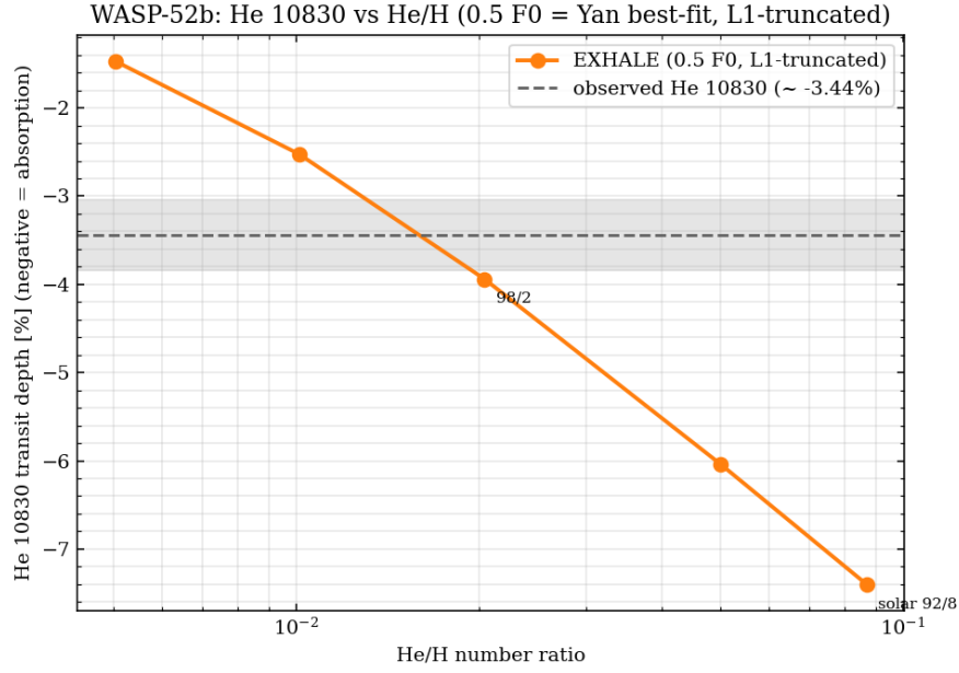
Figure 4: He 10830 line-center transit depth (negative = absorption) vs. He/H number ratio ( 0.5 F_0 , L_1 -truncated). The dashed line and gray band are the observed depth ( -3.44 \pm 0.4\% ). The model crosses the observation near H/He \approx 98/2 , confirming the need for a He-depleted atmosphere.
