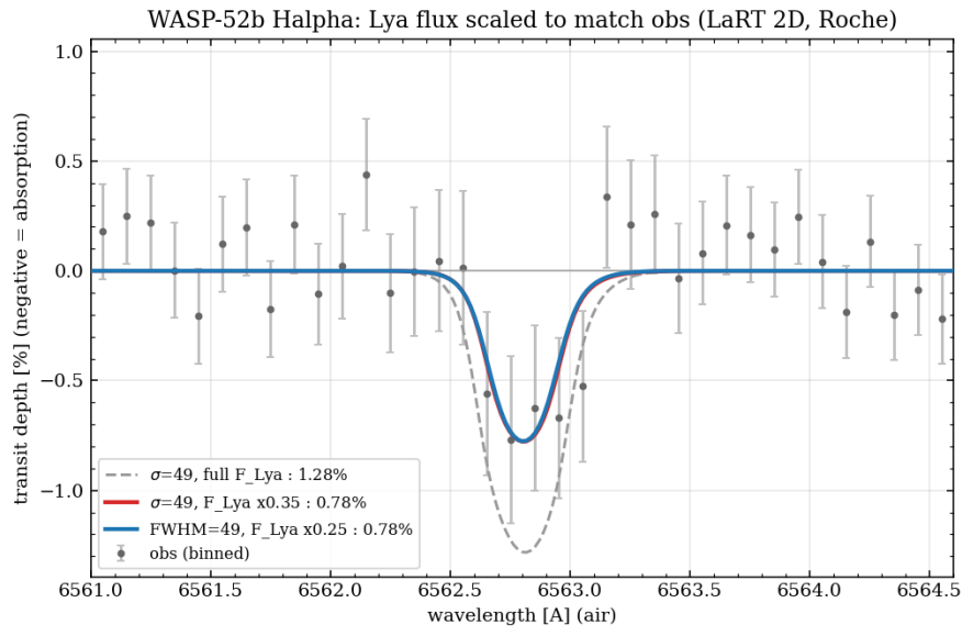
Figure 8: H \alpha with the incident Ly \alpha flux scaled to match the data (LaRT 2-D, L_1 /Roche). Red: \sigma = 49 profile at F_{\text{Ly}\alpha} \times 0.35 (−0.78%); blue: FWHM= 49 profile at \times 0.25 (−0.78%); both match the observed \sim -0.77\% bump and nearly coincide. Dashed grey: \sigma = 49 at full proxy flux (−1.28%). Only L_{\text{Ly}\alpha} is rescaled; the atmospheric structure and LaRT P_\alpha(\rho, z) are unchanged.
