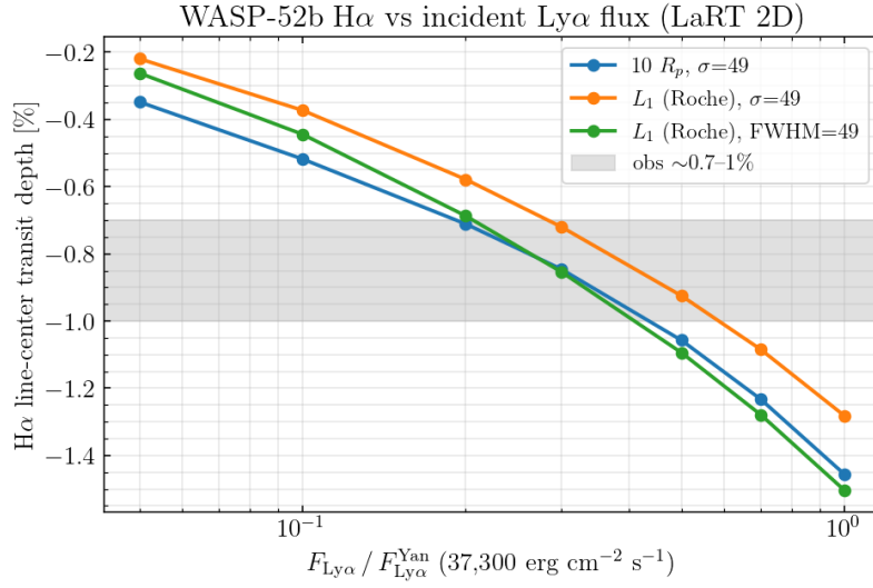
Figure 7: H \alpha line-center transit depth (negative = absorption) vs. the incident Ly \alpha flux scale (LaRT 2-D, L_{\text{Ly}\alpha} rescaled only). The shaded band is the observed depth (−1 to −0.7%); both domains cross it below the EP Eri-proxy value.
