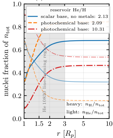
(a) elemental fractions
