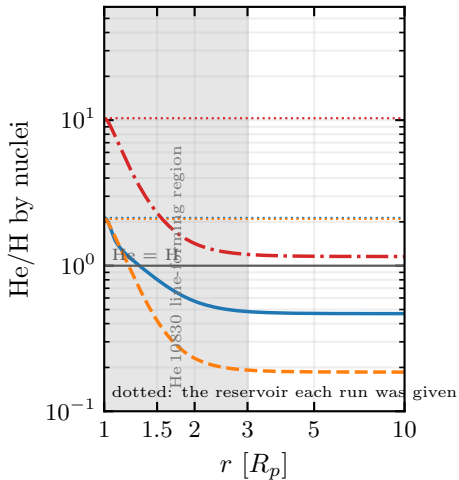
(b) helium against hydrogen
