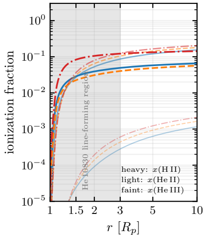
(c) ionization state
