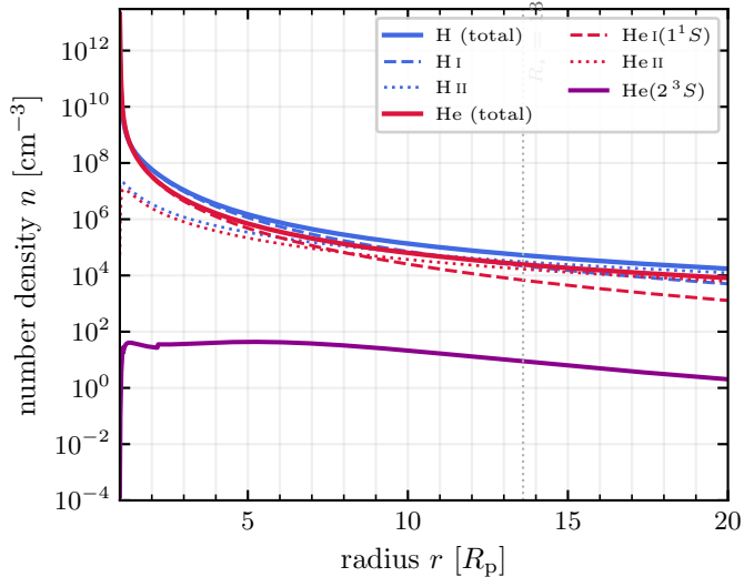
(a) H and He number densities ( K_{zz} = 3.6 \cdot 10^9 , He/H = 2.13)
