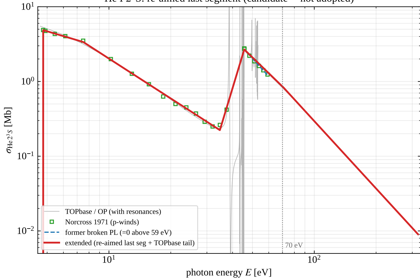
He I 2^3S : re-aimed last segment (candidate -- not adopted)
