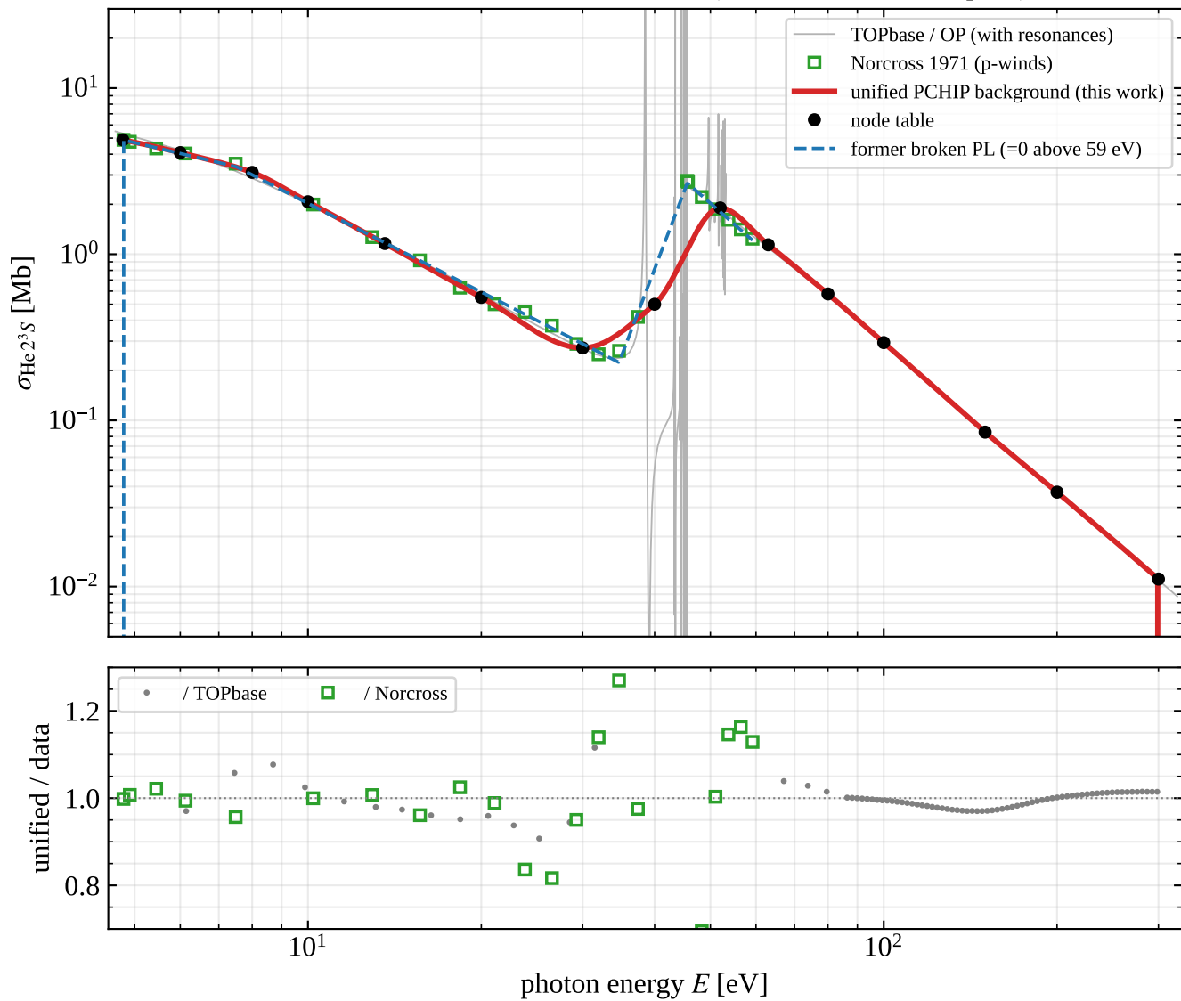
He I 2^3\text{S} : unified PCHIP node table (candidate -- not adopted)
