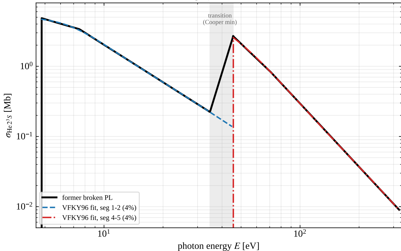
He I 2^3S : two VFKY96 wings (ADOPTED -- now in cross_sec.f90)
