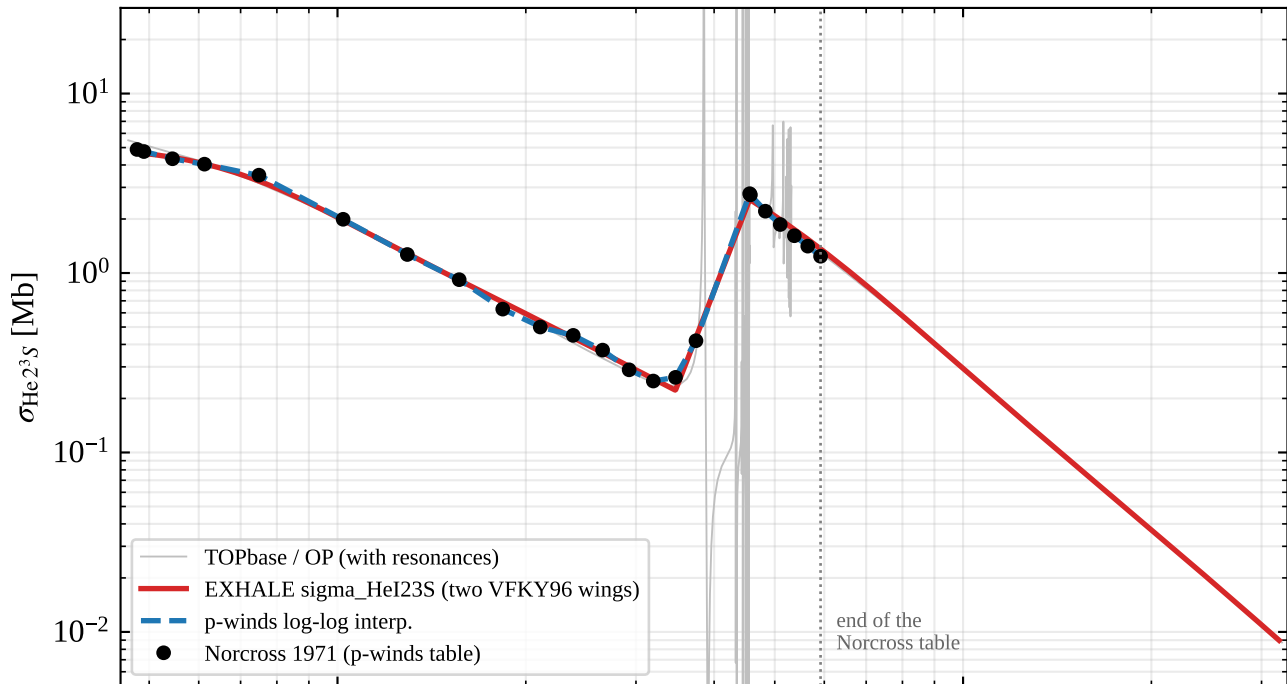
He I 2^3\text{S} photoionization: EXHALE vs p-winds (Norcross 1971)
