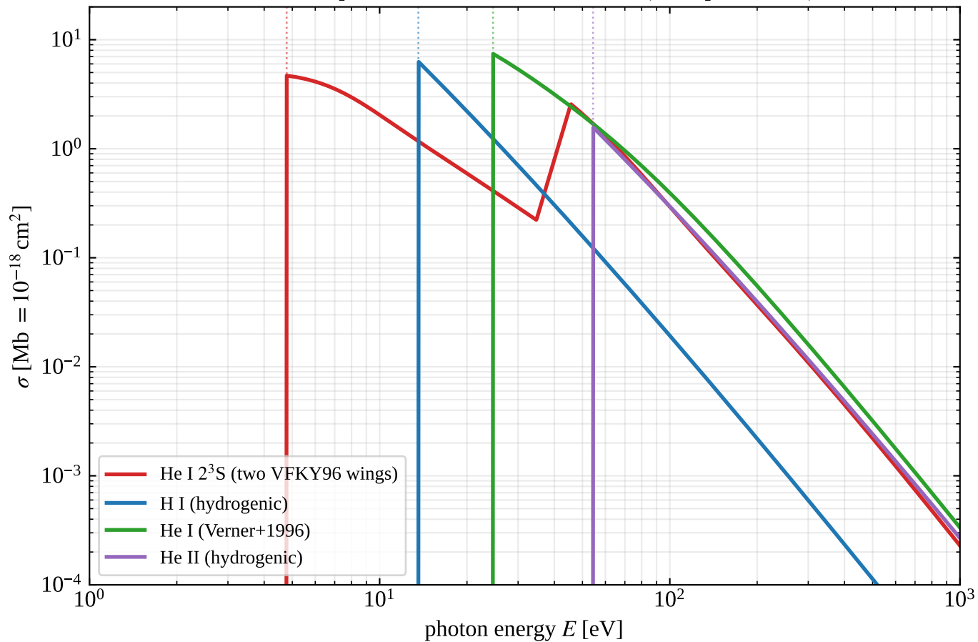
EXHALE photoionization cross sections (as implemented)
