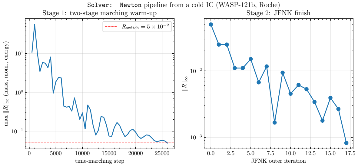
Figure 1: The Solver: Newton route from a cold IC (WASP-121b, Roche). Left: maximum steady residual \max \|R\|_\infty over the mass, momentum, and energy equations during the two-stage (Reconstruction scheme: PLM+WENO3) marching warm-up; the dashed line is the legacy residual hand-off threshold R_{\text{switch}} = 5 \times 10^{-2} used when this figure was produced (the current default keys the hand-off on du < 10^{-2} instead, at a comparable point on the warm-up). Right: residual vs. JFNK outer iteration during the Newton finish, down to \text{Resid tol} ( 10^{-5} ).
