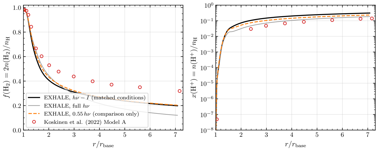
Figure 4: Fraction of H nuclei bound in H_2 (left) and ionized fraction of hydrogen (right); black h\nu - I , gray full h\nu , dashed 0.55 h\nu .
