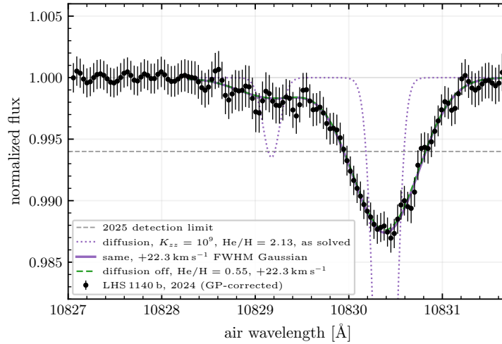
Figure 7: The EW-matched diffusive solution as solved (dotted purple, its core running below the plotted range) and convolved with the 22.3 \text{ km s}^{-1} FWHM Gaussian that reproduces the measured width (solid purple), against the measurement; the diffusion-off \text{He}/\text{H} = 0.55 curve at its own matched kernel (dashed green) is repeated from Fig. 4. The two broadened curves are indistinguishable — their kernels differ by 0.01 \text{ km s}^{-1} . All curves are shifted by the same v_{\text{wind}} = +2.26 \text{ km s}^{-1} .
