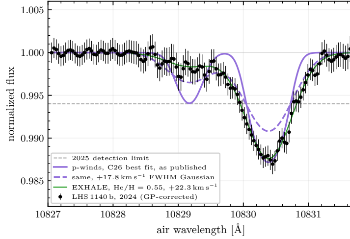
Figure 8: The C26 p-winds best fit as published (solid purple) and convolved with the 17.8 \text{ km s}^{-1} FWHM Gaussian that reproduces the measured width (dashed purple), against the measurement; the EXHALE \text{He}/\text{H} = 0.55 curve at its own matched kernel ( 22.3 \text{ km s}^{-1} , thin green) is repeated from Fig. 4. Broadened to the observed width, the p-winds curve passes above the red core: the width is matched and the depth is not. All curves are shifted by the same v_{\text{wind}} = +2.26 \text{ km s}^{-1} .
