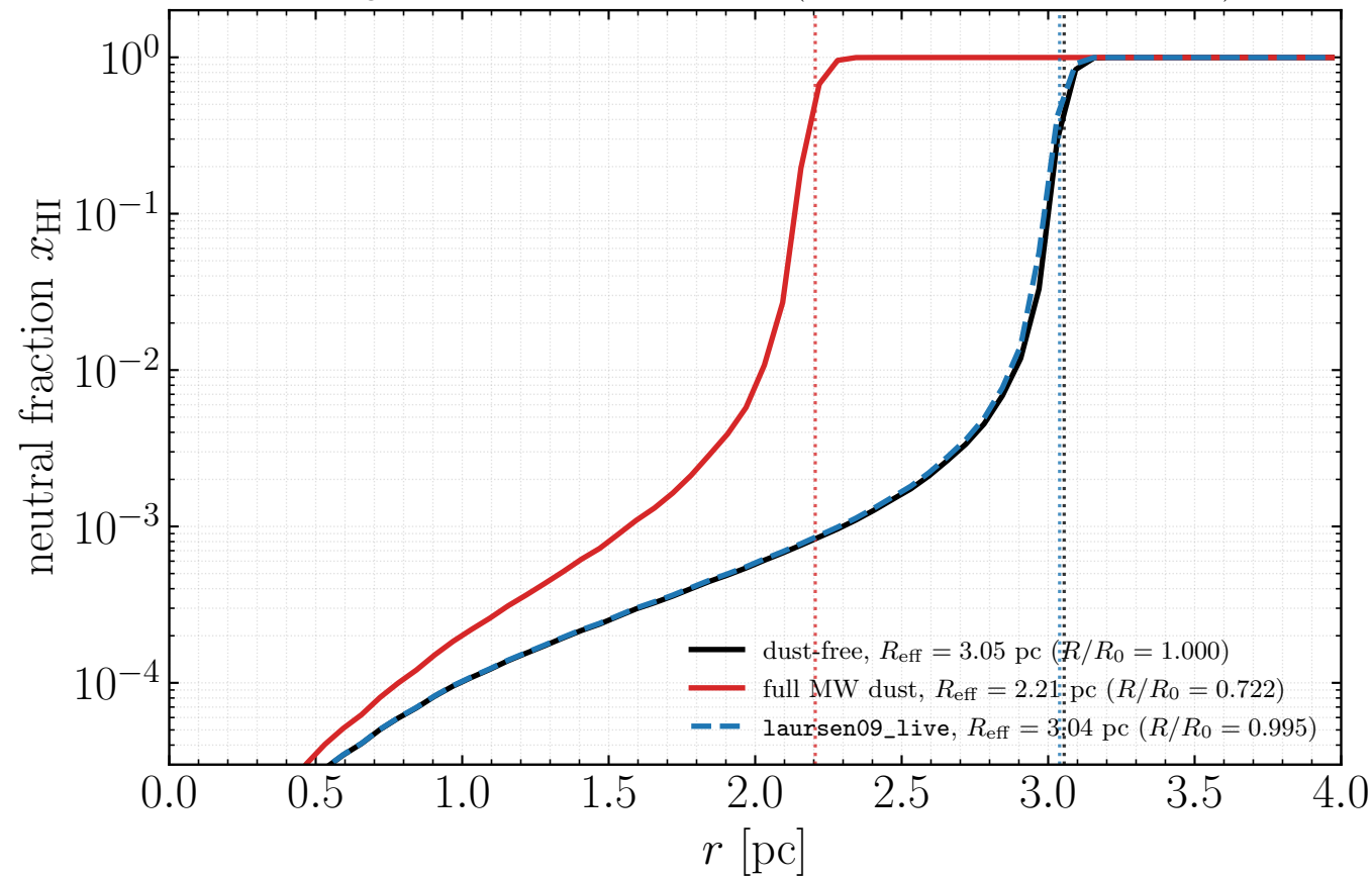
H II region size versus dust treatment ( n_{\text{H}} = 100 \text{ cm}^{-3} , Q_{\text{H}} = 10^{49} \text{ s}^{-1} )
