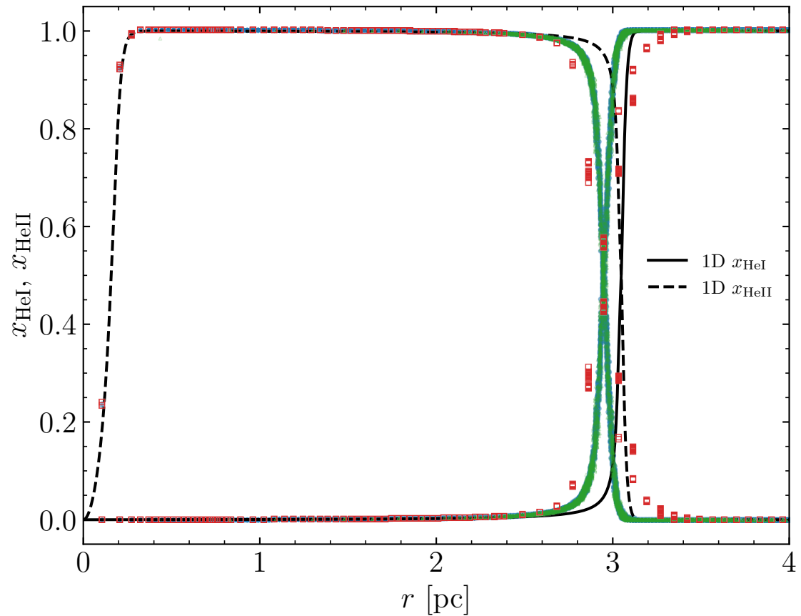
He ionization structure
