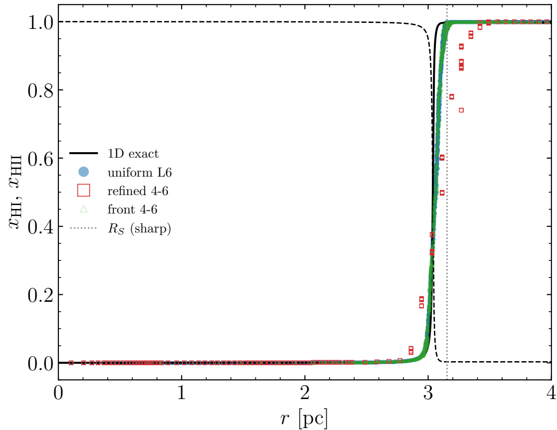
H ionization structure
