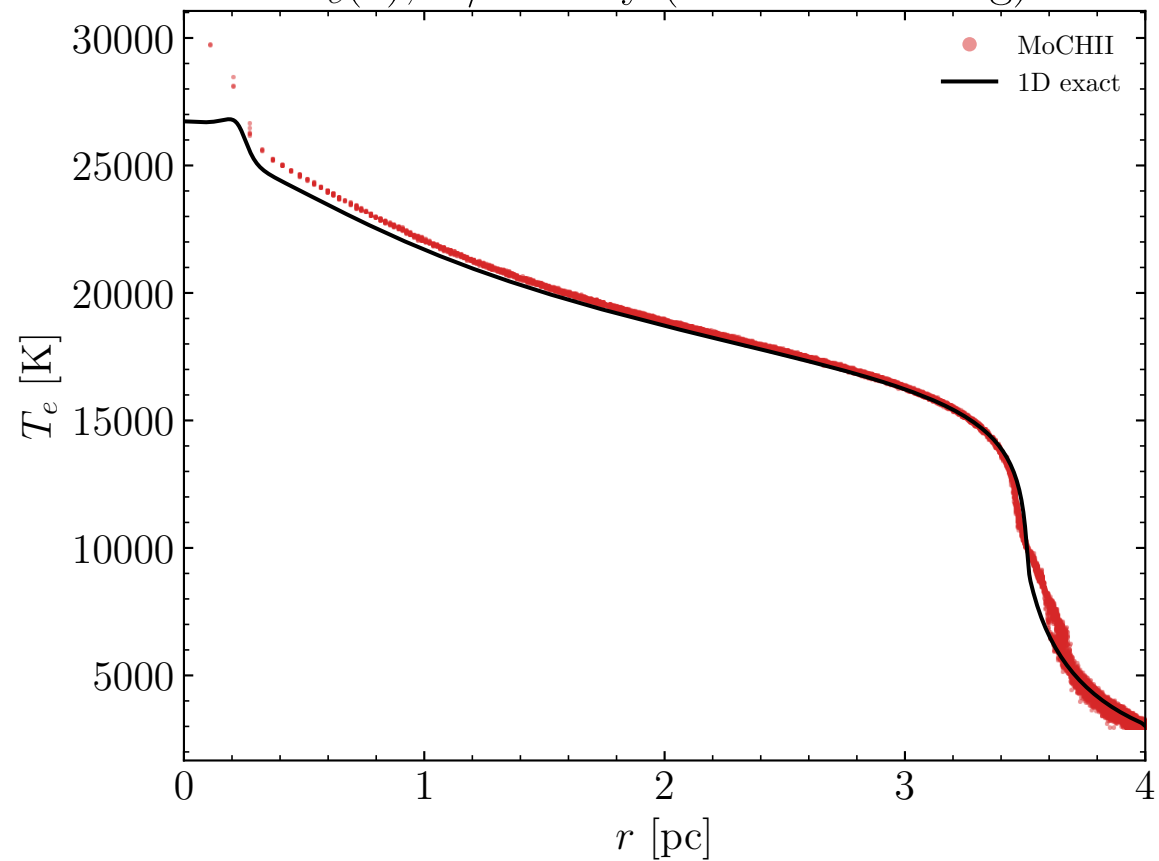
T_e(r) , H/He only (no metal cooling)
