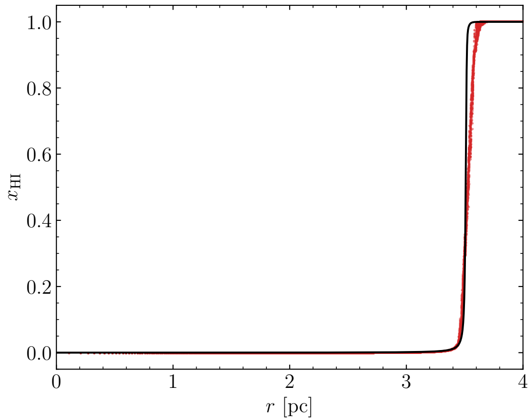
H ionization with thermal balance
