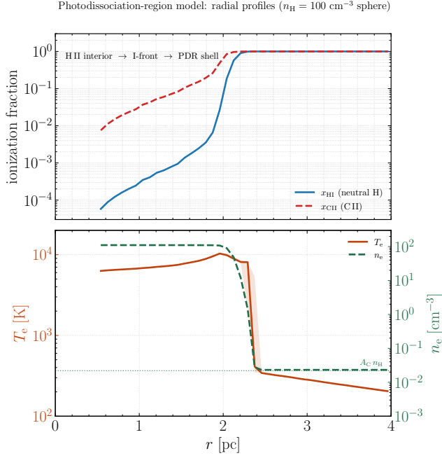
Figure 13. Radial structure of the PDR test: the neutral fraction, electron temperature, and electron density as a function of radius. Inside the front the gas is fully ionized; beyond it the electron density drops to the carbon-dominated value and the temperature settles to a PDR equilibrium above the floor.
