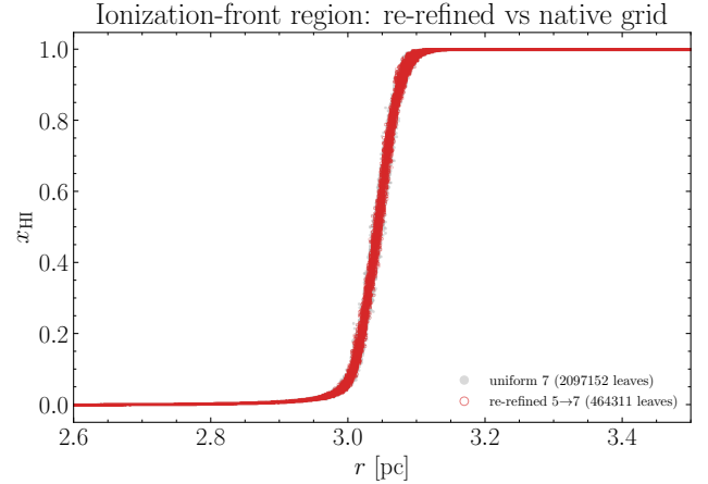
Figure 8. Re-refinement test: the front profiles of the re-refined 5 → 7 octree and the native uniform level-7 grid overlaid exactly, at 4.5× fewer cells.
