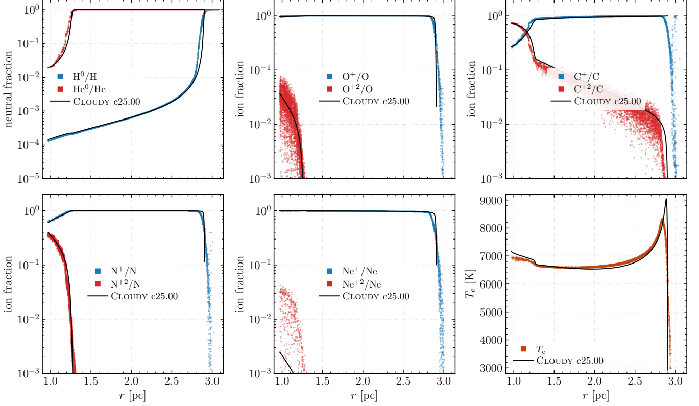
Figure 15. Lexington HII20 benchmark, in the panel layout of K. Wood et al. (2004), their Figure 2; conventions as in Figure 14. Ne^{+2} is confined within 1.4 pc, and C^{+3} stays below the plotted range and carries no series. This is the same run as the MoCHII column of Table 5. At 20 kK the helium-ionizing photons are so few that helium is neutral beyond 1.4 pc. The continuous-energy treatment nonetheless preserves the weak C^{+2} tail outside that helium transition. Black lines are CLOUDY c25.00 on the same model, from the unmodified c25.00 deck tsuite/auto/hii_coolstar.in behind the C25 column of Table 5. CLOUDY stops on its own criterion at 2.91 pc, short of the outer radius of the MoCHII shell, so its curves end there, and its final near-vertical fall is the recombination front itself, resolved in zones far finer than a MoCHII cell.
