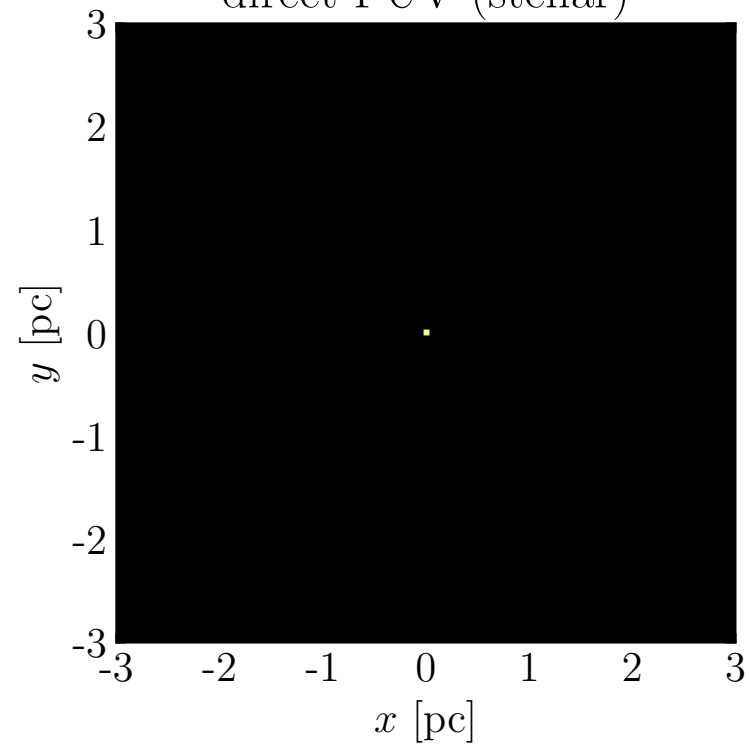
direct FUV (stellar)
