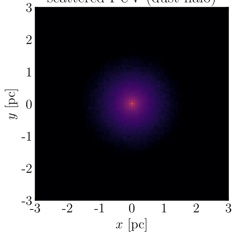
scattered FUV (dust halo)
