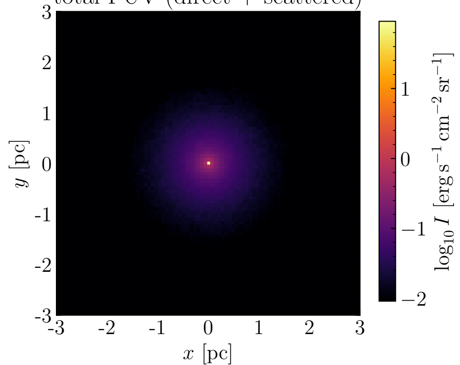
total FUV (direct + scattered)
