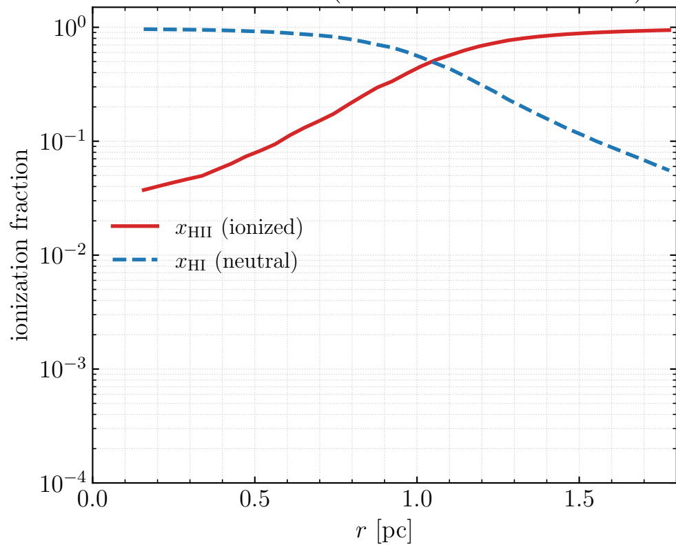
radial structure (field enters from r = R )
