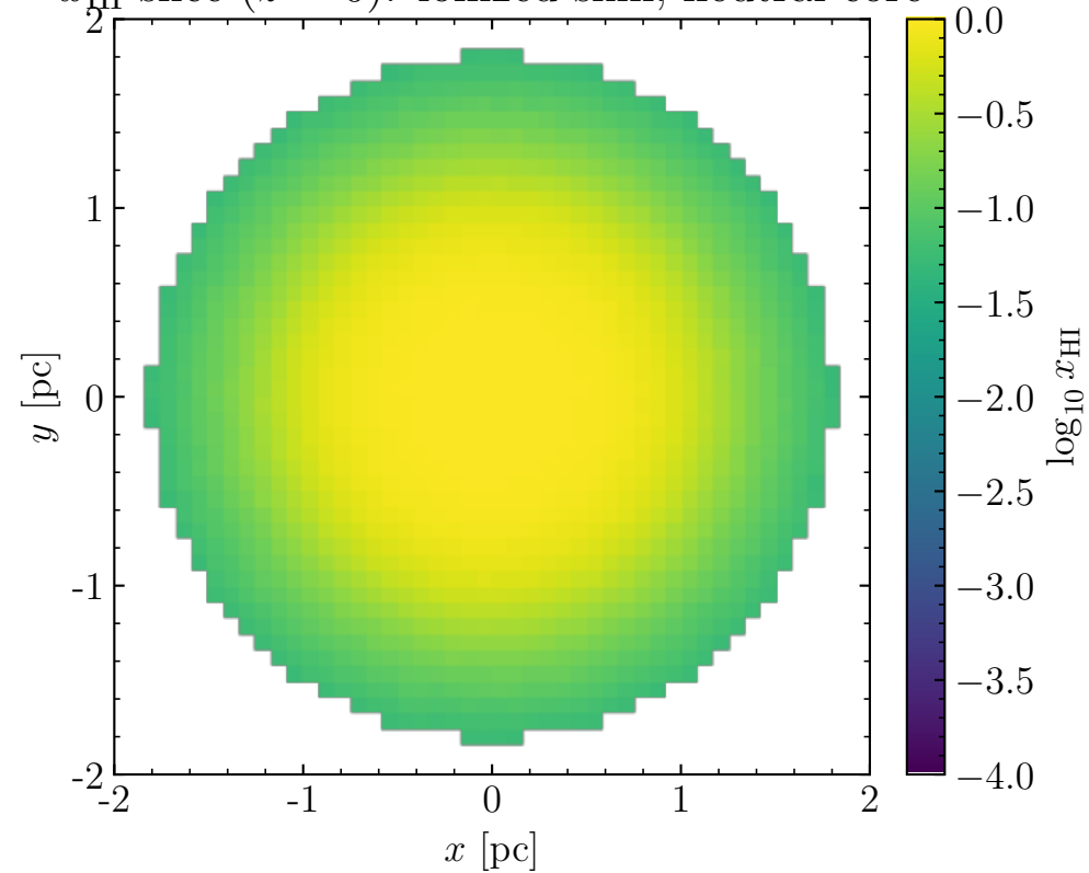
x_{\text{HI}} slice ( z = 0 ): ionized skin, neutral core
