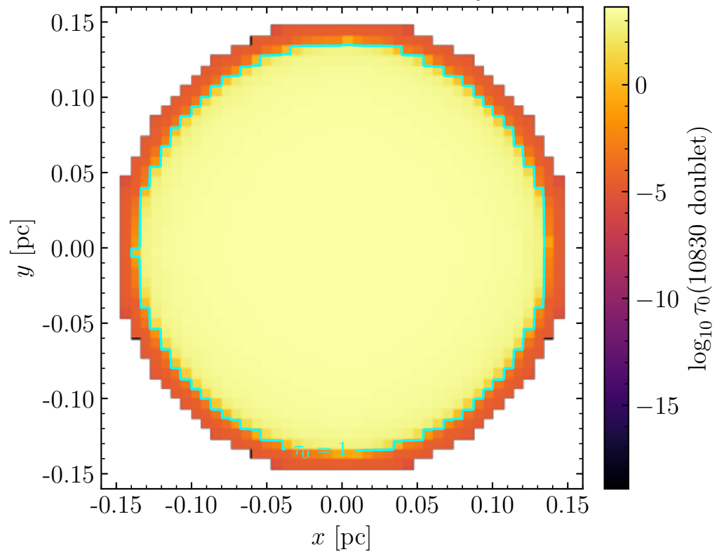
10830 \text{ \AA} line-center \tau_0
