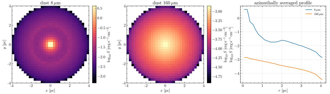
Figure 12. Dust emission at 8 and 160 \mu\text{m} from the stochastic SEDust solve, as two-dimensional projection maps of the surface brightness (left, middle) with their azimuthally averaged radial profiles (right). The short wavelength is centrally peaked (warm inner dust), falling by 3.5 dex across the sphere, while the far-infrared profile is far flatter (1.6 dex), the projected signature of the dust temperature gradient.
