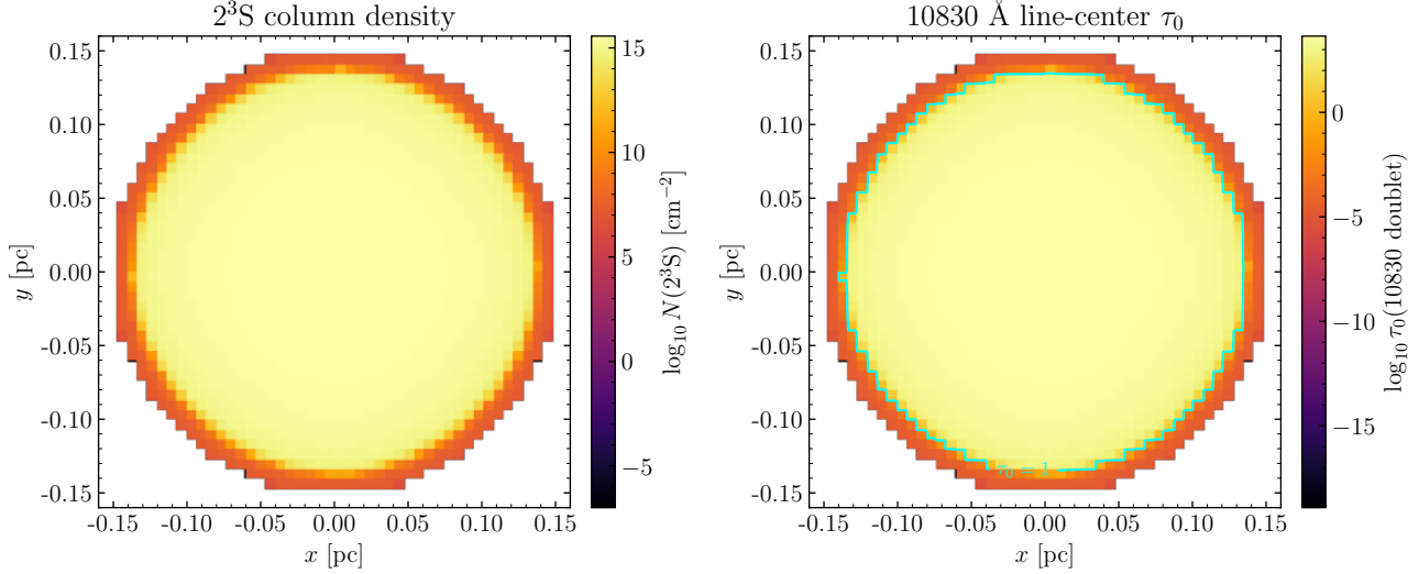
Figure 4. The He I 2^3\text{S} metastable diagnostic for a dense compact example ( n_{\text{H}} = 10^4 \text{ cm}^{-3} , R = 0.15 \text{ pc} , T_e = 10^4 \text{ K} ), as line-of-sight projection maps. Left: the 2^3\text{S} column density. Right: the 10830 \text{ Å} line-center optical depth \tau_0 of the blended J' = 1, 2 doublet, with the \tau_0 = 1 contour (cyan); the core is optically thick, where the optically-thin diagnostic breaks down.
