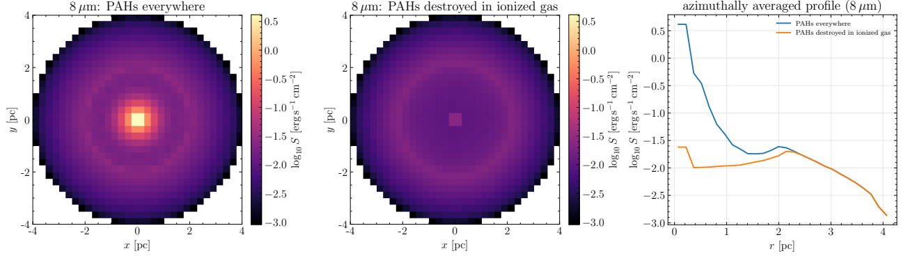
Figure 11. Stochastic dust emission at 8 \mu\text{m} with the ionization-dependent PAH share. The first two panels are two-dimensional projection maps (the emissivity integrated along the line of sight into a surface brightness) sharing one brightness scale. Left: PAHs surviving everywhere, giving a centrally peaked image. Middle: PAHs destroyed in the ionized interior ( x_{\text{HII}} -weighted survival). Right: the azimuthally averaged radial profiles of both maps. Destroying the PAHs removes the central peak and leaves a broad limb-brightened annulus just inside the ionization front at r \simeq 2.1 pc, visible in the profile as a local maximum a factor 1.9 above the depressed interior.
