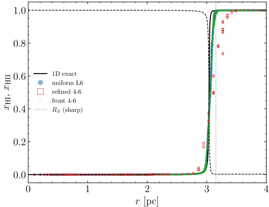
H ionization structure
