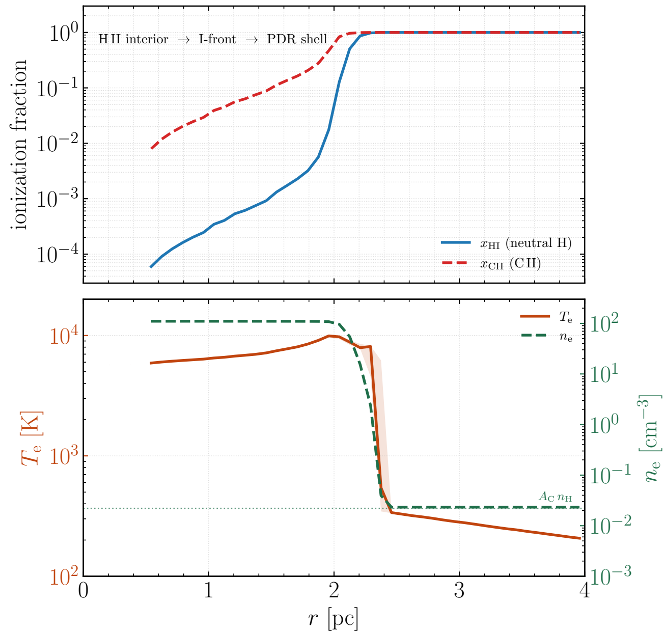
Photodissociation-region model: radial profiles ( n_{\text{H}} = 100 \text{ cm}^{-3} sphere)
