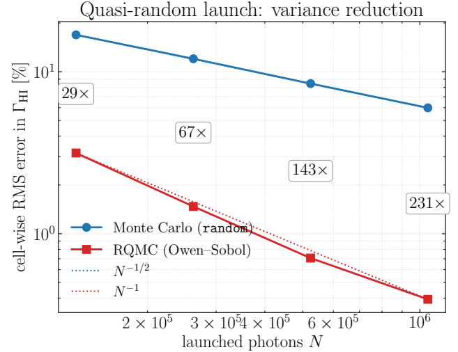
Figure 2. Quasi-random photon launching. Cell-wise root-mean-square error in \Gamma_{\text{HI}} on the fixed-state analytic-attenuation test, as a function of the launched photon count N , for the ordinary Monte Carlo ( random ) and Owen-scrambled Sobol (RQMC) launches, with the N^{-1/2} and N^{-1} reference slopes. The boxed labels give the effective-photon gain (the variance ratio) at each N , which grows with N as the two slopes diverge.
