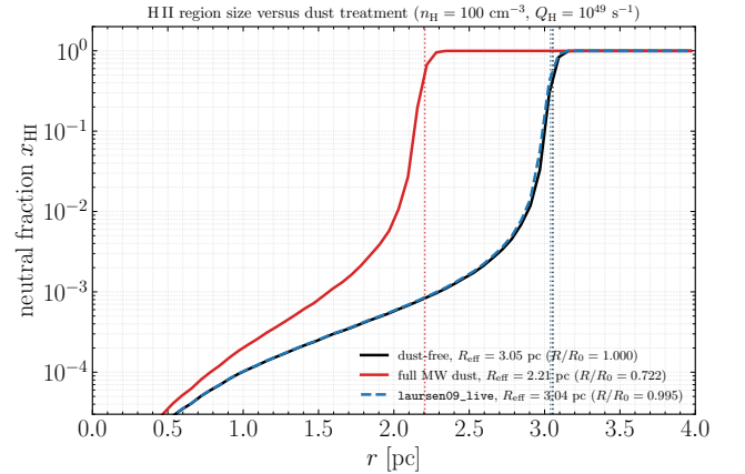
Figure 10. H II region size versus dust treatment: the radial neutral-fraction profile x_{\text{HI}}(r) for the dust-free, full MW dust, and laursen09_live runs of the same Strömgren configuration ( n_H = 100 \text{ cm}^{-3} , Q_H = 10^{49} \text{ s}^{-1} , T_\star = 4 \times 10^4 \text{ K} , case B). Dotted vertical lines mark each effective ionized radius R_{\text{eff}} . Full MW dust pushes the ionization front inward to R/R_0 = 0.722 , while the live ionization-dependent dust vanishes in the ionized interior and recovers the dust-free size ( R/R_0 = 0.996 ).
