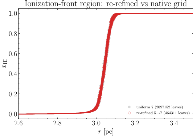
Figure 8. Re-refinement test: the front profiles of the re-refined 5 \rightarrow 7 octree and the native uniform level-7 grid overlies exactly, at 4.5\times fewer cells.
