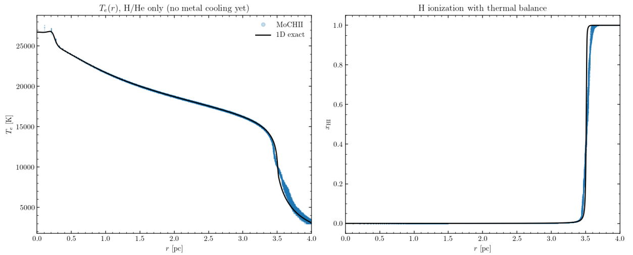
Figure 3: Thermal gate: T_e(r) and x_{\text{HI}}(r) with the thermal balance, against the 1D exact reference.
