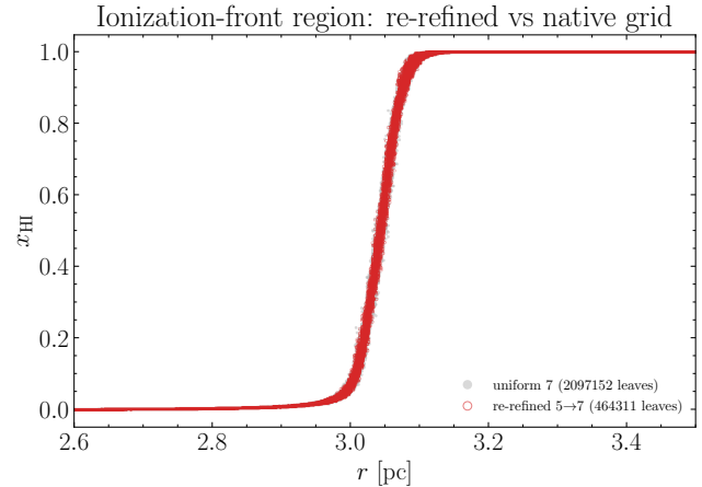
Figure 8. Re-refinement test: the front profiles of the re-refined 5 \rightarrow 7 octree and the native uniform level-7 grid overlaid exactly, at 4.5 \times fewer cells.
