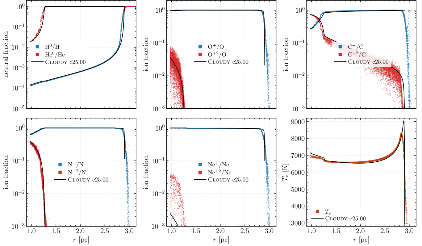
Figure 15. Lexington HII20 benchmark, in the panel layout of K. Wood et al. (2004), their Figure 2; conventions as in Figure 14. \text{Ne}^{+2} is confined within 1.4 pc, and \text{C}^{+3} stays below the plotted range and carries no series. This is the same run as the MoCHII column of Table 5. At 20 kK the helium-ionizing photons are so few that helium is neutral beyond 1.4 pc. The continuous-energy treatment nonetheless preserves the weak \text{C}^{+2} tail outside that helium transition. Black lines are CLOUDY c25.00 on the same model, from the unmodified c25.00 deck tsuite/auto/hii_coolstar.in behind the C25 column of Table 5. CLOUDY stops on its own criterion at 2.91 pc, short of the outer radius of the MoCHII shell, so its curves end there, and its final near-vertical fall is the recombination front itself, resolved in zones far finer than a MoCHII cell.
