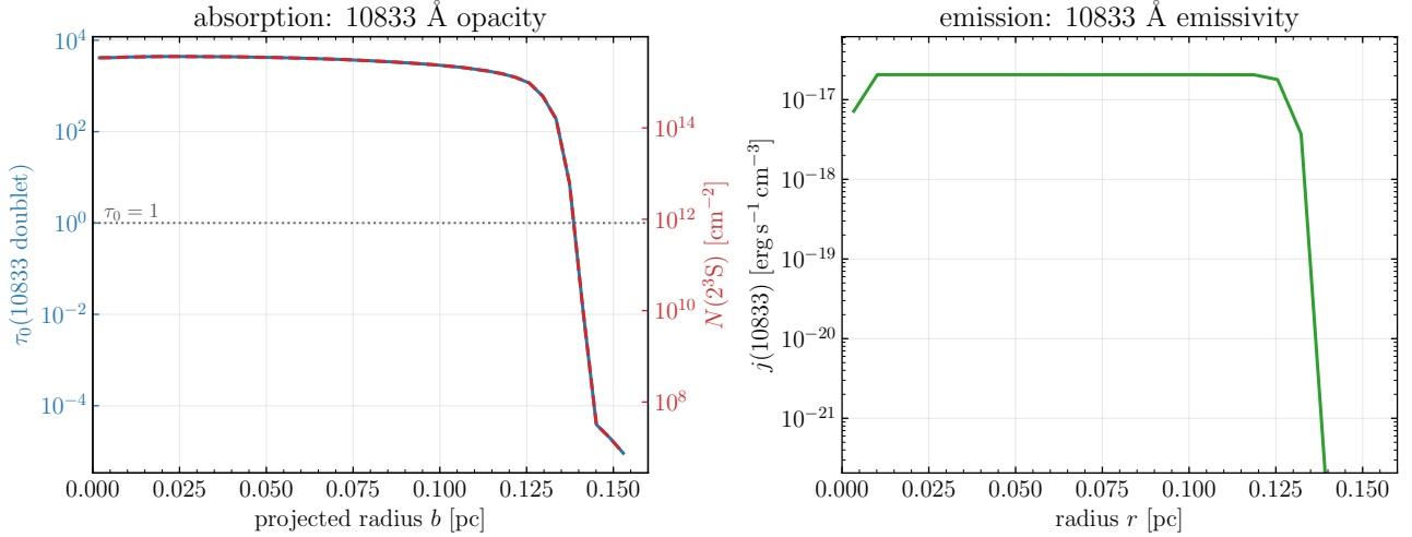
Figure 4. The He I 2^3\text{S} metastable diagnostic for a dense compact example ( n_{\text{H}} = 10^4 \text{ cm}^{-3} , R = 0.15 \text{ pc} , T_e = 10^4 \text{ K} ), as radial profiles of the two sides of the same 2^3\text{S} – 2^3\text{P} transition. Left, absorption: the 10833 Å line-center optical depth \tau_0 of the blended J' = 1, 2 doublet against projected radius (left axis) with the 2^3\text{S} column density on the right axis. Both are line-of-sight integrals, and at the fixed T_e of this run the Doppler width is constant, so the two are strictly proportional and the right axis is the conversion of the left; the curves overlap. The region is optically thick inside b = 0.139 \text{ pc} , where the optically-thin diagnostic breaks down. Right, emission: the 10833 Å emissivity against radius, from the R. L. Porter et al. (2012) He I block of the emissivity file.
