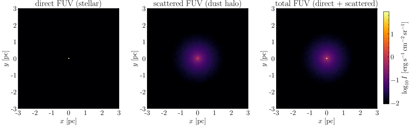
Figure 3. Peel-off synthetic imaging of a dusty, FUV-illuminated H II region with a central star, in the FUV channel. Left: the direct stellar image, an attenuated point source. Center: the dust-scattered halo, the observer-oriented contribution. Right: their sum, the synthetic observation. All three panels share one logarithmic scale of the specific intensity I integrated over the channel’s band, so the extended scattered halo is directly comparable to the compact direct source.
